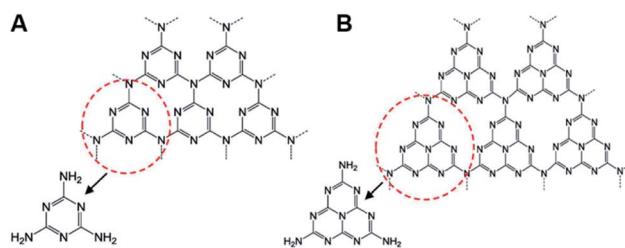
Fig. 1 (A) Triazine and (B) tri- s -triazine as the basic structural units of g\text{-C}_3\text{N}_4 . Reproduced from ref. 34 with permission from The American Chemical Society.
