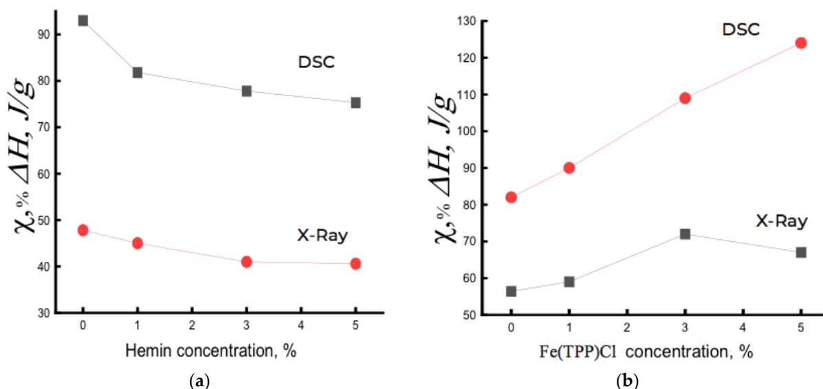
Figure 3. Dependence of the degree of crystallinity \chi and enthalpy of melting \Delta H on the composition of the mixed composition of (a) PHB/hemin and (b) PHB/ \text{Fe}(\text{TPP})\text{Cl} .
