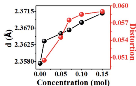
Fig. 10 MYAS:xDy 3+ : changes in bond length and twist of Y/Mg(1)O 6 .
