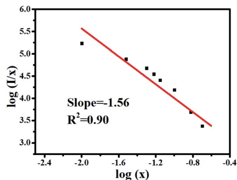
Fig. 9 Graph of \log(I/x) and \log(x) for MYAS:xDy 3+ .
