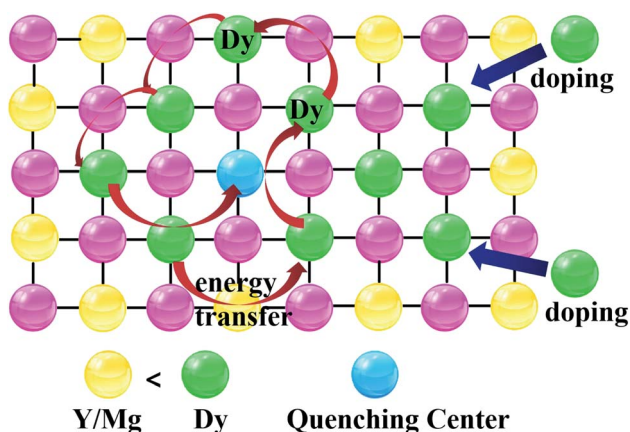
Fig. 8 Schematic diagram of concentration quenching process of Dy 3+ .
