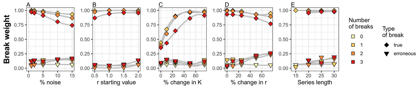
Fig 2. Average break weight of break points detected under varying parameterization conditions. Average weights of break points identified by the Dynamic Shift Detector algorithm reflecting true parameterization conditions (diamonds) or erroneous breaks suggested by the algorithm (triangles) under varied A) noise (in the form of normally distributed error), B) starting values of the r parameter, C) percent changes in the K parameter, D) percent changes in r , and E) simulated time series length. Sets of 0, 1, 2 and 3 break points were randomly generated from within the set of possible values, and 250 datasets were simulated for each scenario. In each panel, other variables (that were not being varied) were held constant at their base values (i.e., noise = 2%; starting value of r = 2; change in r = \pm 25\% ; change in K = \pm 75\% ; time series length = 20 years). Trends within a set of scenarios (grey lines) are illustrated with a third-order GAM smoothing line.
