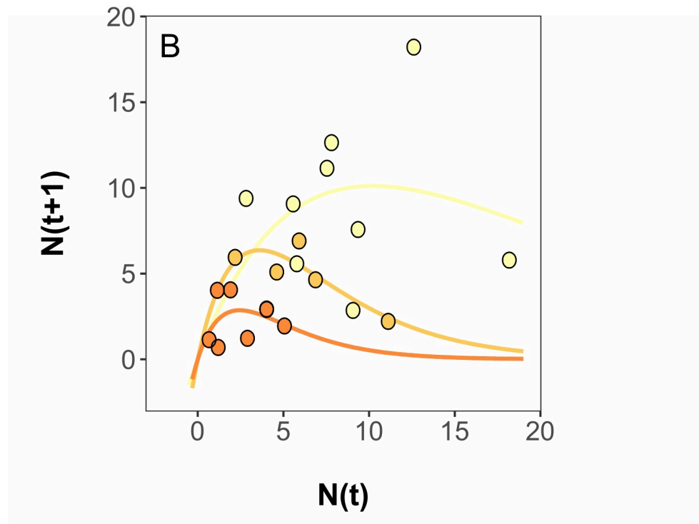
Fig 4. Dynamic Shift Detector breaks and Ricker model fits for a species of conservation concern. Population data documenting the area occupied by monarch butterflies in their winter habitat in central Mexico from 1995–2017. A) Time series data showing the total area occupied by overwintering monarchs each year in December. Vertical blue lines indicate years in which dynamic shifts occurred, as estimated by the Dynamic Shift Detector algorithm. B) Ricker fits of time series data segments. Butterfly art by D. Descouens and T.M. Seeseey, used under a CC-BY 3.0 license.
