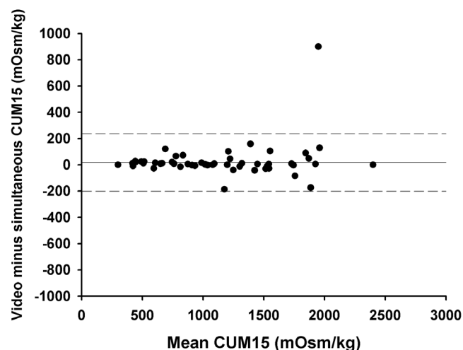
Figure 3 The Bland-Altman plot for CUM15, the index that was used to express cough sensitivity in hypertonic saline challenge. The difference between video vs. simultaneously counted CUM15 is plotted against the mean of the respective index. The solid horizontal line represents the mean difference between the two counting methods and the dashed lines the 95% limits of agreement.
