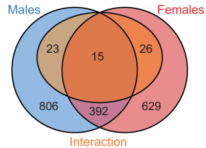
Fig. 3 Venn diagrams showing the overlap of genes differentially expressed in response to cold treatment in males (blue) and females (red). Genes with a significant sex-by-treatment interaction are shown in orange, showing that the majority of genes differentially expressed in males and females do not have significant sex-by-treatment interactions (color figure online).
