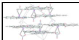
Fig. 2. The packing diagram viewed down the c axis. The dashed lines represent intermolecular C—H...O interactions.
