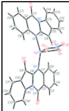
Fig. 1. The molecular structure of the title compound showing 30% probability displacement ellipsoids.
