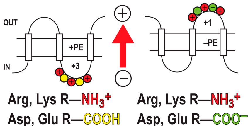
Figure 6. PE and the positive inside rule. In the left panel a cytoplasmic domain is shown containing a mixture of negative and positive amino acids. PE suppresses or neutralizes the presence of negative residues (yellow circles), which increases the effective positive charge potential, thus favoring cytoplasmic retention of the domain. In the absence of PE (right panel) negative residues (green circles) exert their full potential, resulting in translocation of the domain with a lower effective net positive charge. The proton motive force (arrow) positive outward determines domain directional movement depending on the domain effective net charge as influenced by the lipid environment.
