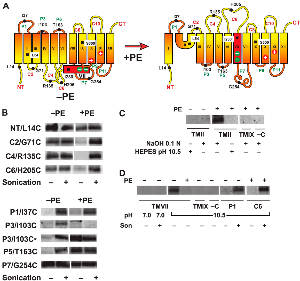
Figure 1. PE-induced post-insertion topological reorganization of LacY. (A) Change in topology of LacY assembled in -PE cells (left panel; Bogdanov et al., 2002) after post-assembly synthesis of PE (right panel; this paper) in strain AT2033. Rectangles define the TMs (Abramson et al., 2003) oriented with the cytoplasm above the figure. TMs (roman numerals), extramembrane domains (P for periplasmic and C for cytoplasmic as oriented in +PE cells), N terminus (NT), and C terminus (CT) are indicated. The locations of negatively charged and positively charged residues involved in salt bridges between TMs are indicated. The locations and names of amino acids substituted by cysteine and used for SCAM analysis are indicated near circles (extramembrane) or squares (within TMs). TMVII is indicated in a periplasmic location (left) and a membrane-inserted location (right). (B–D) AT2033 cells without (–) or with (+) sonication were treated with MPB as described in Materials and methods. Labeling was performed on samples either after initial assembly of LacY in -PE cells ( -PE , with IPTG induction but before addition of \alpha Tc ) or after removal of IPTG and induction of PE synthesis ( +PE ) for 3 h (maximum PE level) during logarithmic growth ( OD_{600} increased from 0.4 to 1–1.4). Western blotting was used to detect biotinylation of diagnostic cysteines that were accessible to MPB; domain and/or substitution positions are indicated. Images are horizontal strips of the LacY (33 kD) position. See Materials and methods for details of image acquisition. (B) MBP labeling was performed at pH 7.5 except for P3/I103C*, where labeling was done at pH 10.5. (C and D). Labeling pH is indicated, and the cysteine substitutions in TMII, TMVII, and TMIX were L54C, I230C, and S300C, respectively. The substitutions in P1 and C6 are those noted in (B), and “–C” refers to cysteine-less LacY. Sonication of the TMVII samples from -PE and +PE cells followed by SCAM analysis at pH 10.5 gave the same result as shown in lanes 3 and 4 from the left in D, respectively (not depicted).
