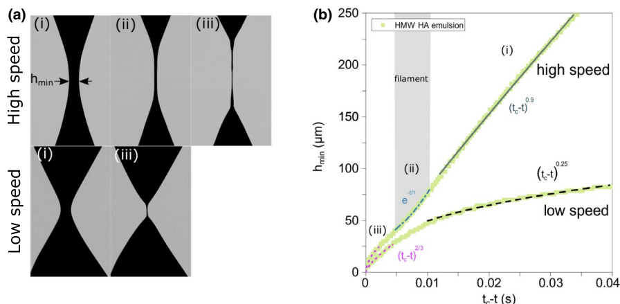
FIGURE 3 (a) Photographs of the neck break-up dynamics of HMW HA emulsions at a high speed (10 mm/s) and low speed (10 \mu\text{m}/\text{s} ).
