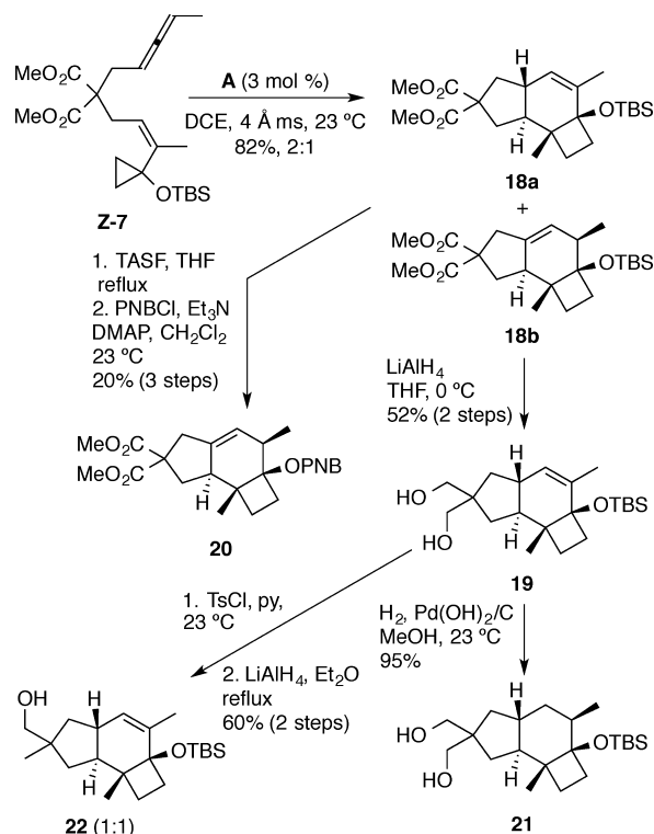
Scheme 5. Gold(I)-Catalyzed Cyclization of Z-7
