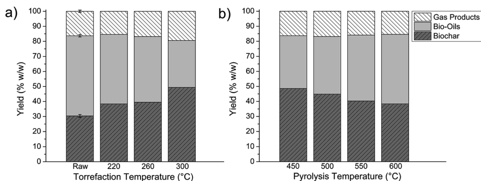
Fig. 3 Yields of pyrolytic char, oil, and gas products from tobacco residues for varying (a) torrefaction and (b) pyrolysis temperatures.
