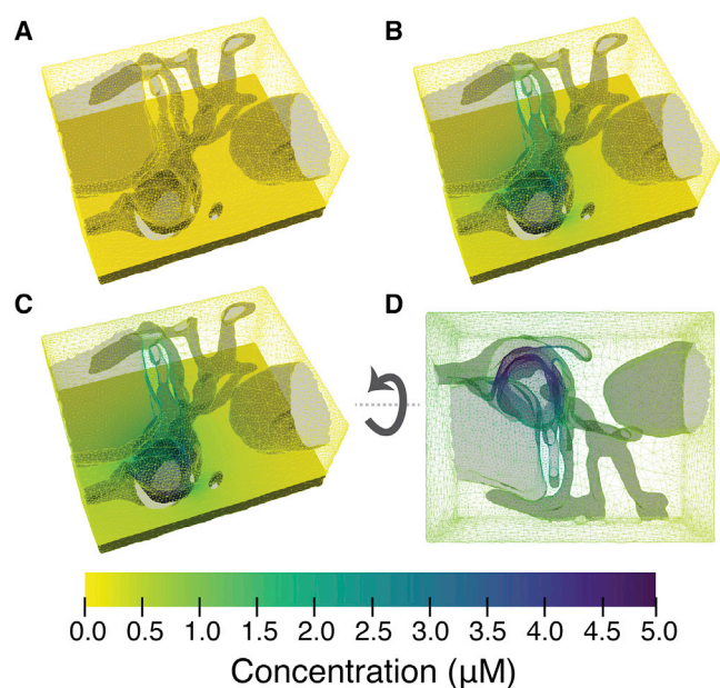
FIGURE 3 Snapshots of molecular diffusion in the CRU geometry. In (A), the initial condition is shown; in (B), 200 \mu\text{s} is shown; in (C), 400 \mu\text{s} is shown; in (D), 5000 \mu\text{s} is shown. The molecules can be trapped in locally confined regions leading to microdomains with locally increased concentrations. To see this figure in color, go online.
