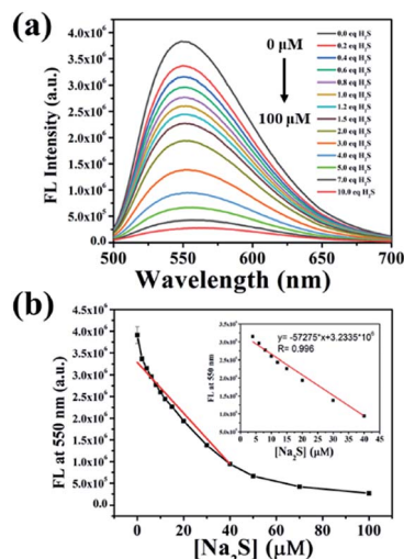
Fig. 1 (a) Fluorescence spectra of 10 \mu\text{M} NP-biotin upon the addition of 0–100 \mu\text{M} under the excitation of 480 nm; (b) the relationship between fluorescence intensity of NP-biotin at 550 nm and \text{Na}_2\text{S} concentration in the range of 0–100 \mu\text{M} (inset: linearity between the fluorescence intensity of NP-biotin at 550 nm and \text{Na}_2\text{S} concentration in the range of 0–40 \mu\text{M} ).
