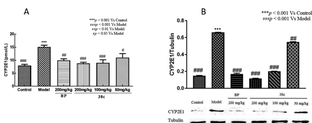
Fig. 6 Effect of compound 38c pretreatment on (A) serum and (B) liver homogenates CYP2E1 protein levels in mice treated with 10 mL kg -1 CCl 4 . Data are expressed as means ± SD ( n = 8). *** P < 0.001 compared to control. # P < 0.05, ## P < 0.01, ### P < 0.001 compared to CCl 4 model mice.
