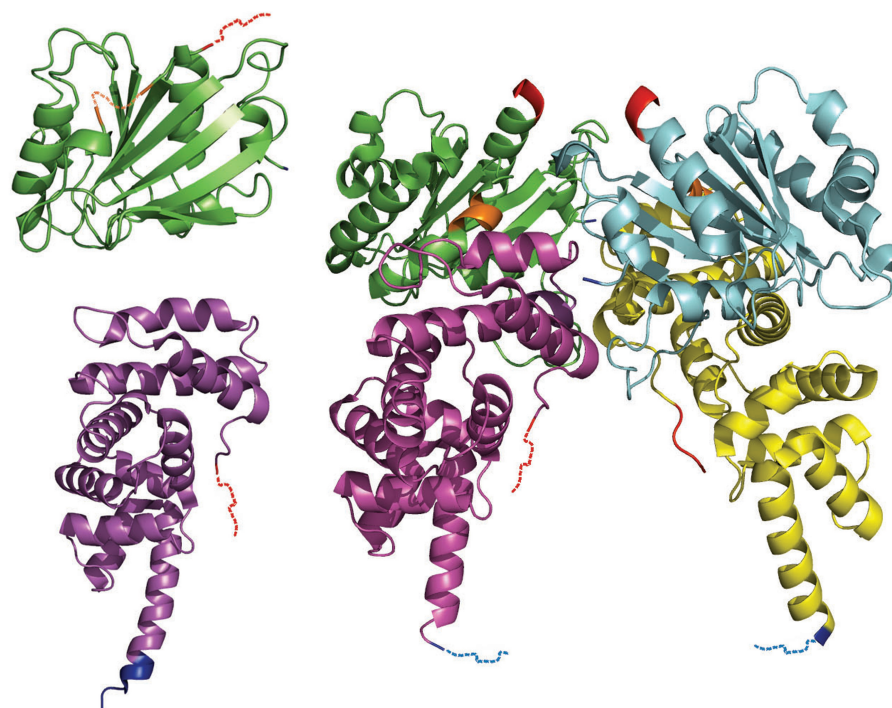
Figure 1. ADP-ribosylation factor (green and blue chains) and exchange factor ARNO (magenta and yellow chains) in unbound (left; PDB entries 1RRF and 1R8M, correspondingly) and bound (right; PDB entry 1R8Q) forms. Blue, red and orange dashed lines correspond to disordered regions at N-terminus, at C-terminus and in the central part of protein chains, correspondingly.
