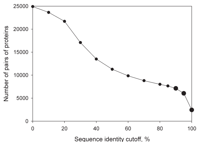
Figure 2. Dependence of the number of complex-single pairs on the sequence identity cutoff. There are 2448, 6051 and 7129 single-complex pairs at 100, 95 and 90% identity level cutoffs, respectively.
