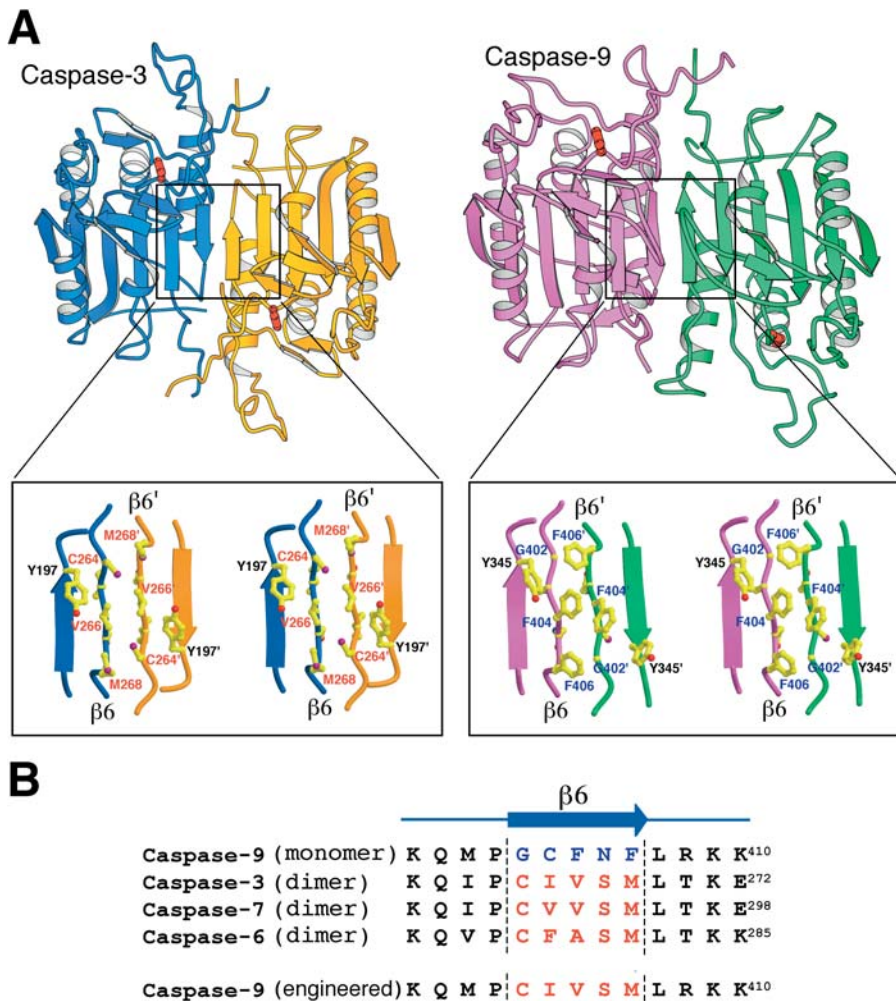
Figure 1. The \beta 6 Strand Is the Major Determinant for the Dimerization of Caspases
