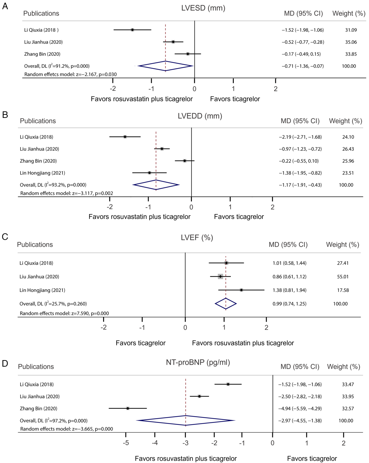
Figure 4. Forest plot of the comparison of cardiac function between rosuvastatin plus ticagrelor and ticagrelor monotherapy. Pooled analysis of (A) LVESD, (B) LVEDD, (C) LVEF and (D) NT-proBNP. Data are presented as MD with 95% CI. LVESD, LV end-systolic diameter; LVEDD, LV end-diastolic diameter; LVEF, left ventricular ejection; NT-proBNP, N-terminal pro-B-type natriuretic peptide; MD, mean difference; CI, confidence interval.
