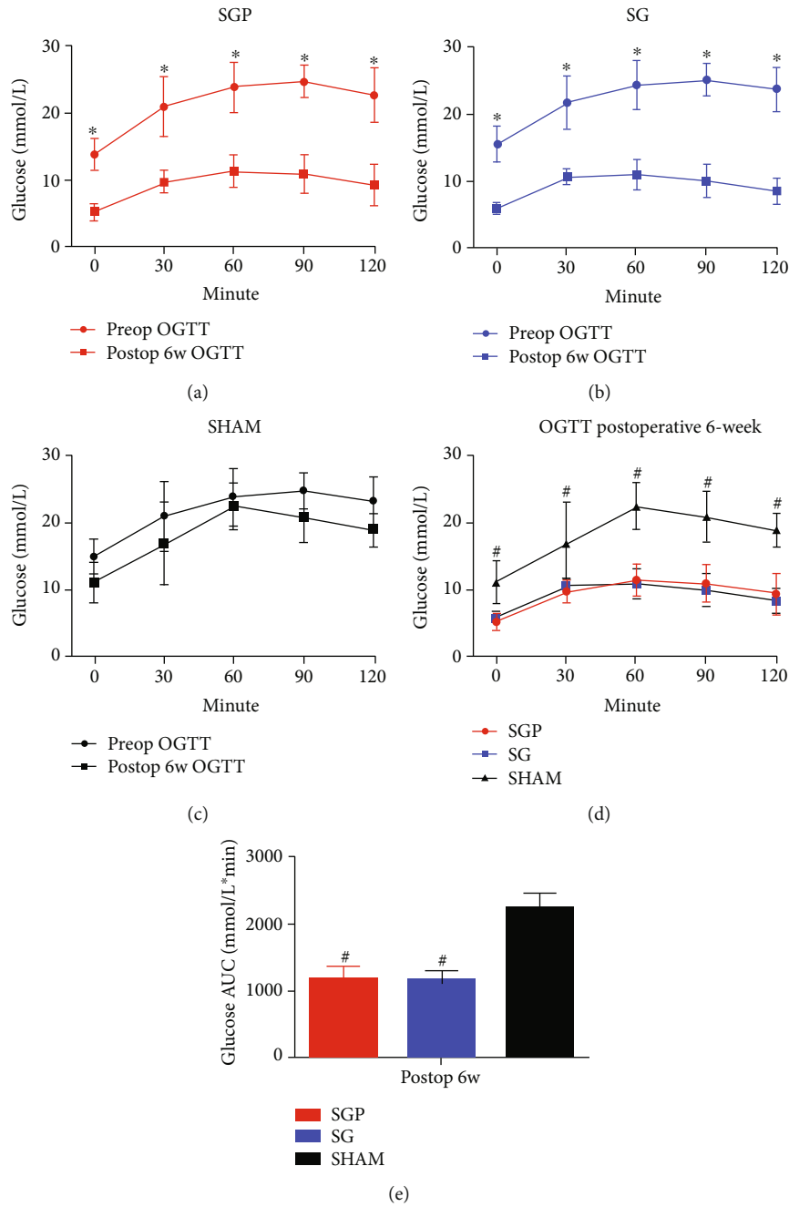
FIGURE 3: OGTT results preoperatively (preoperative) and postoperatively (postoperative): (a) SGP, (b) sleeve gastrectomy (SG), and (c) SHAM. Group comparison at postoperative level: (d) OGTT. (e) Glucose AUC. * indicates significant difference ( p < 0.05 ). #Significant compared with SHAM ( p < 0.05 ).
