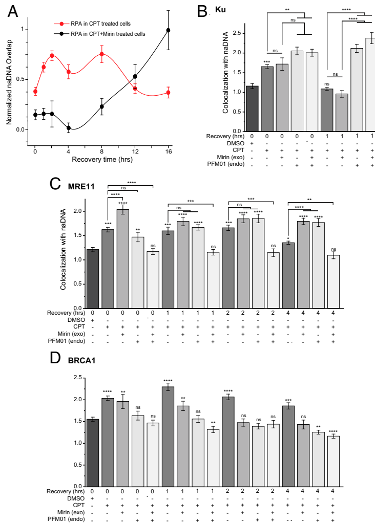
Fig. 6. MRE11 nuclease inhibition using Mirin and PFM01 completely abrogates resection at DSBs, causing delayed repair and apoptosis even after removal of Mirin. (A) Kinetic trace of RPA colocalization with naDNA 0 to 16 h after 1 h of CPT treatment in combination with Mirin (black trace) or with a DMSO control (red). Adapted with permission from ref. 27, which is licensed under CC BY 4.0 . (B) Quantification of Ku association with repair foci in control cells, cells treated with CPT, both CPT + Mirin, both CPT + PFM01, and with CPT + Mirin + PFM01. (C) Quantification of MRE11 association with repair foci in control cells, cells treated with CPT, both CPT + Mirin, both CPT + PFM01, and with CPT + Mirin + PFM01. (D) Quantification of BRCA1 association with repair foci in control cells, cells treated with CPT, both CPT + Mirin, both CPT + PFM01, and with CPT + Mirin + PFM01. Controls are shown for comparison. DMSO signifies dimethyl sulfoxide controls. Student's t test results show significance of difference between CPT-only and CPT + Mirin treatments at indicated times post-CPT. SEs are shown. ns shows P > 0.05 ; *P < 0.05 ; **P < 0.01 ; ***P < 0.001 ; ****P < 0.0001 .
