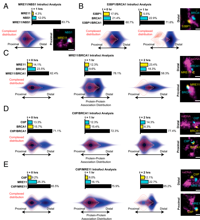
Fig. 4. The spatial organization of NBS1, 53BP1, MRE11, BRCA1, and CtIP demonstrates high levels of colocalization at the same repair foci with dynamic spatially proximal and distal arrangements. (A) Analysis of the internal organization of MRE11 and NBS1 costained and colocalized with naDNA after 1 h of 100 nM CPT treatment. MRE11/NBS1 shows a high level of colocalization at repair foci with a minor fraction (12.0%) MRE11 only (cumulative bar graph). Colocalized MRE11 and NBS1 have a strongly proximal association distribution at 0 h, indicative of closely associated proteins. (B) Analysis of the internal organization of 53BP1 and BRCA1 costained and colocalized with naDNA at 0 and 1 h after 1 h of 100 nM CPT treatment; 53BP1/BRCA1 shows a high level of colocalization at repair foci with minor fractions (5 to 25%) demonstrably MRE11-only or 53BP1-only foci (cumulative bar graph). Colocalized 53BP1 and BRCA1 have a moderately distal association distribution at 0 h that increases in separation at 1 h. (C) Analysis of the internal organization of MRE11 and BRCA1 costained and colocalized with naDNA at 0, 1, and 2 h after 1 h of 100 nM CPT treatment. MRE11/BRCA1 shows a high level of colocalization at repair foci with minor fractions (9 to 24%) demonstrably MRE11-only or BRCA1-only foci (cumulative bar graph). Colocalized MRE11 and BRCA1 have a predominantly proximal association distribution at 0 h, both proximal and distal subpopulations at 1 h, and a predominantly distal distribution by 2 h. (D) Analysis of the internal organization of CtIP and BRCA1 costained and colocalized with naDNA at 0, 1, and 2 h after 1 h of 100 nM CPT treatment. BRCA1/CtIP shows a similarly high degree of colocalization across time points and even smaller fractions (<8 to 16%) as CtIP-only and BRCA1-only foci. Colocalized CtIP and BRCA1 are predominantly proximal in their association distribution across all times with a persistent population of distal, uncomplexed species. (E) Analysis of the internal organization of MRE11 and CtIP costained and colocalized with naDNA at 0, 1, and 2 h after 1 h of 100 nM CPT treatment. CtIP/MRE11 also shows a high degree of colocalization and minor fractions (8 to 26%) of CtIP-only and MRE11-only foci. Colocalized CtIP and MRE11 initially displayed almost equal fractions in distal and proximal arrangements before a shift toward a more proximal distribution at 1 h and then, toward a predominantly distal distribution at 2 h. In all images, the overlaid red contour map outline shows the modeled distribution of closely associated proteins. Representative distal and proximal foci are also shown. (Scale bars: 250 nm.)
