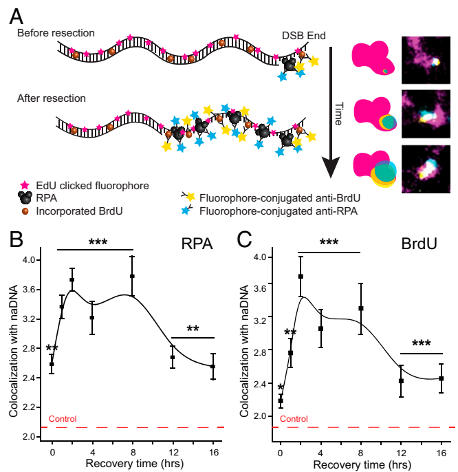
Fig. 2. Quantification of RPA and BrdU overlap signals with naDNA shows resection progression. (A) A schematic model showing labeling for RPA and ssDNA as resection progresses. (B) Kinetic trace of RPA colocalization with naDNA 0 to 16 h after 1 h of 100 nM CPT treatment. (C) Kinetic trace of ssDNA (detected as undenatured BrdU) colocalization with naDNA 0 to 16 h after 1 h of 100 nM CPT treatment. SEs are shown. * P < 0.05 based on two-sample Student's t test comparing damaged time point data with control undamaged cell colocalization levels; ** P < 0.01 based on two-sample Student's t test comparing damaged time point data with control undamaged cell colocalization levels; *** P < 0.001 based on two-sample Student's t test comparing damaged time point data with control undamaged cell colocalization levels.
