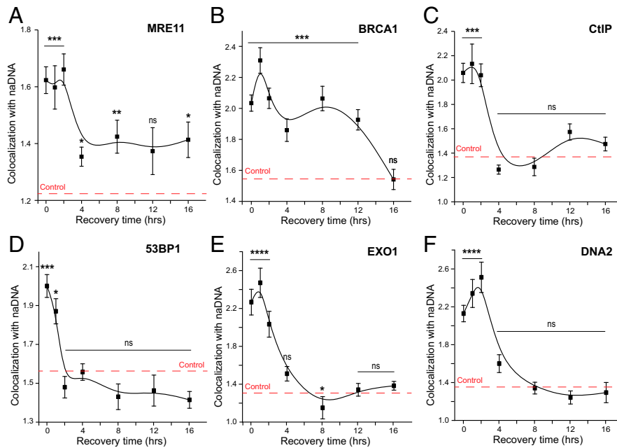
Fig. 3. MRN, BRCA1, and CtIP associate with DSBs to orchestrate resection during the first 2 h of repair. (A) Kinetic trace of MRE11 colocalization with naDNA 0 to 16 h after 1 h of 100 nM CPT treatment. (B) Kinetic trace of BRCA1 colocalization with naDNA 0 to 16 h after 1 h of 100 nM CPT treatment. (C) Kinetic trace of CtIP colocalization with naDNA 0 to 16 h after 1 h of 100 nM CPT treatment. (D) Kinetic trace of 53BP1 colocalization with naDNA 0 to 16 h after 1 h of 100 nM CPT treatment. (E) Kinetic trace of EXO1 colocalization with naDNA 0 to 16 h after 1 h of 100 nM CPT treatment. (F) Kinetic trace of DNA2 colocalization with naDNA 0 to 16 h after 1 h of 100 nM CPT treatment. SEs are shown. ns shows P > 0.05 based on two-sample Student's t test against undamaged cell colocalization levels. *P < 0.05 based on two-sample Student's t test against undamaged cell colocalization levels; **P < 0.01 based on two-sample Student's t test against undamaged cell colocalization levels; ***P < 0.001 based on two-sample Student's t test against undamaged cell colocalization levels; ****P < 0.0001 based on two-sample Student's t test against undamaged cell colocalization levels.
