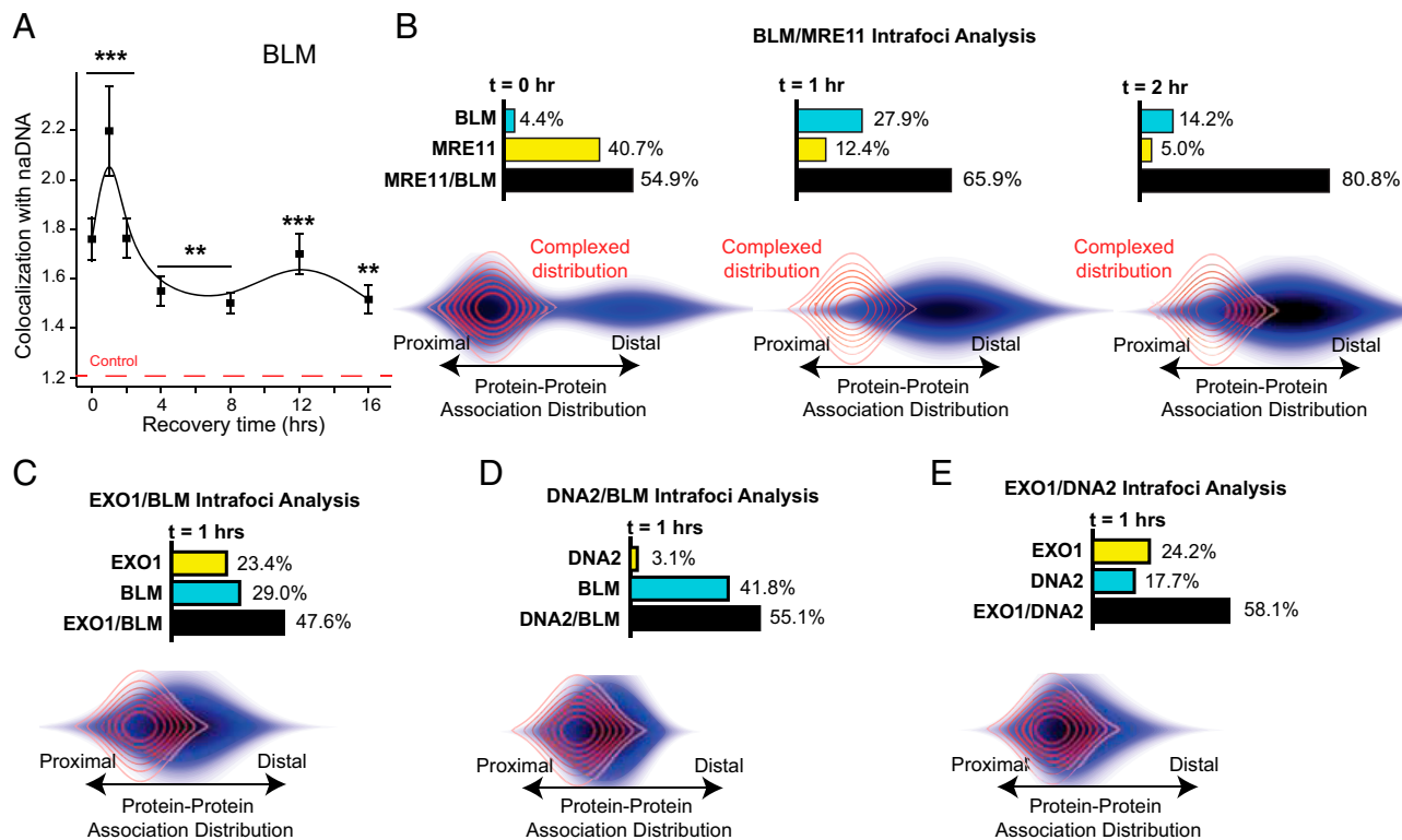
Fig. 5. BLM is involved dynamically with nucleases EXO1, DNA2, and MRE11 during resection. (A) Kinetic trace of BLM colocalization with naDNA 0 to 16 h after 1 h of 100 nM CPT treatment. ^{**}P < 0.01 based on two-sample Student's t test against undamaged cell colocalization levels; ^{***}P < 0.001 based on two-sample Student's t test against undamaged cell colocalization levels. (B) Analysis of the internal organization of MRE11 and BLM costained and colocalized with naDNA 0, 1, and 2 h after 1 h of 100 nM CPT treatment. MRE11/BLM shows a moderate, increasing to high level of colocalization at repair foci, with significant MRE11 only observed at the 0-h time point. Colocalized MRE11 and BLM have a mixed proximal and distal arrangement immediately following damage, indicating both complexed and spatially separated species. At 1 and 2 h, the spatial arrangement indicates separation of MRE11 and BLM. (C) Analysis of the internal organization of EXO1 and BLM costained and colocalized with naDNA 1 h after treatment with 100 nM CPT for 1 h. Significant levels of EXO1/BLM colocalization at damage foci are detected along with EXO1 and BLM localizations independent of each other. Spatially, colocalized EXO1/BLM shows a moderately distal arrangement indicating the predominance of spatial independence. (D) Analysis of the internal organization of DNA2 and BLM costained and colocalized with naDNA 1 h after treatment with 100 nM CPT for 1 h. Significant levels of DNA2/BLM colocalization at damage foci are detected along with BLM localizations independent of DNA2 presence. Minimal DNA2 localization to damage foci is detected independent of BLM, indicating DNA2's dependence on BLM. Spatially, colocalized DNA2/BLM shows a more proximal arrangement compared with EXO1/BLM, indicating increased interaction, although still with some proteins spatially separated within the foci. (E) Analysis of the internal organization of EXO1 and DNA2 costained and colocalized with naDNA 1 h after treatment with 100 nM CPT for 1 h. Significant levels of EXO1/DNA2 colocalization at damage foci are detected along with EXO1 and DNA2 localizations independent of each other. Spatially, colocalized EXO1/DNA2 shows a moderately proximal arrangement similar to DNA2/BLM, indicating some instances of both interaction and spatial separation. SEs are shown.
