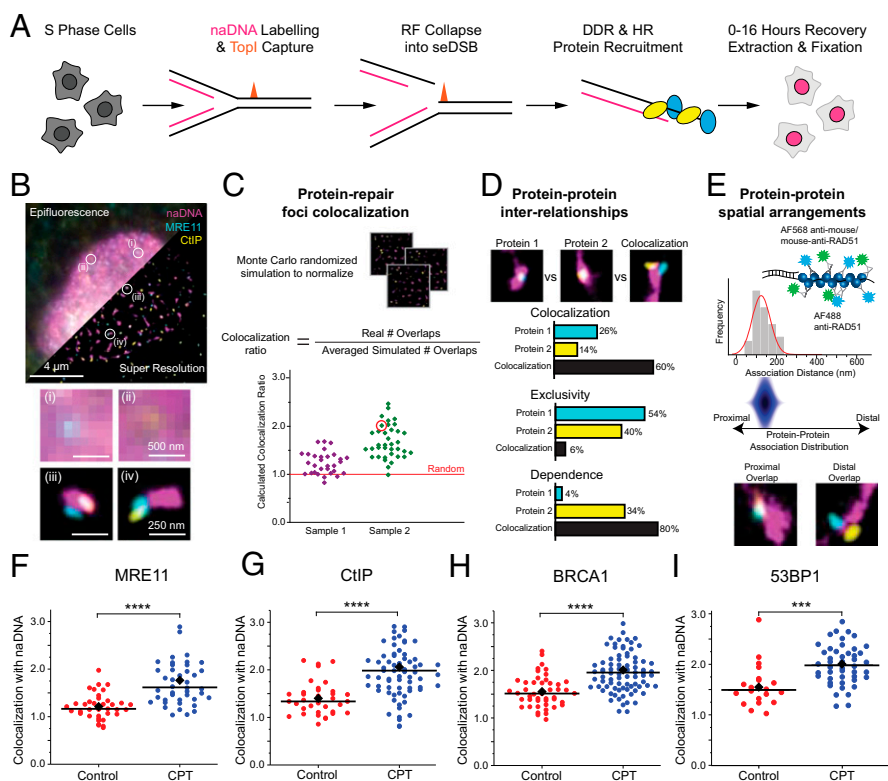
Fig. 1. SR imaging of repair proteins recruited to individual seDSBs in human cells. (A) The experimental protocol used to label and break RFs into seDSBs in order to capture snapshots of the arrivals, accumulations, and departures of repair proteins. TopI, Topoisomerase I; DDR, DNA damage response. (B) Representative epifluorescence (upper left) and SR (lower right) images of a single nucleus damaged and labeled for naDNA (using EdU; magenta), MRE11 (cyan), and CtIP (yellow). (B, i and ii) Representative zoomed-in epifluorescence and (B, iii and iv) SR foci are shown. (Scale bars: i and ii, 500 nm; iii and iv, 250 nm.) (C) Schematic showing the analytical process for quantifying protein colocalization with repair foci by generating Monte Carlo randomized simulation images for each SR nucleus image and then using the number of overlaps in the random simulations to normalize the real data. For each cell, this normalized “colocalization ratio” can be plotted (e.g., one normalized cell value is circled in red) and compared with truly random levels (=1) and with control levels in untreated control cells. (D) The interrelationships between proteins localized to repair foci were further quantified by calculating the percentage of naDNA foci positive for one or both stained proteins. This determined the degree of colocalization between proteins at repair sites, as well as exclusion and dependence relationships. (E) The spatial relationship of pairs of proteins colocalized at repair foci could be determined by measuring the distance between the protein foci centers of mass and generating a histogram. This was then extrapolated to generate a protein–protein association distribution two-dimensional heat map. By staining RAD51 with two different fluorophores, we could model the expected association distribution for proximally associated proteins for comparison with proteins that are distally associated at repair foci. Representative foci show proximal and distal overlaps as observed in dual-stained RAD51 (proximal; magenta: naDNA, cyan/yellow: RAD51) and in MRE11 (cyan) and CtIP (yellow; distal; magenta: naDNA). (F–H) Scatterplots showing quantification of colocalization between (F) MRE11, (G) CtIP, (H) BRCA1, and (I) 53BP1 with naDNA in untreated control cells and cells treated with 100 nM CPT for 1 h. Black bars depict medians, and diamonds show the means. *** P < 0.001 in a two-sample Student’s t test; **** P < 0.0001 in a two-sample Student’s t test.
