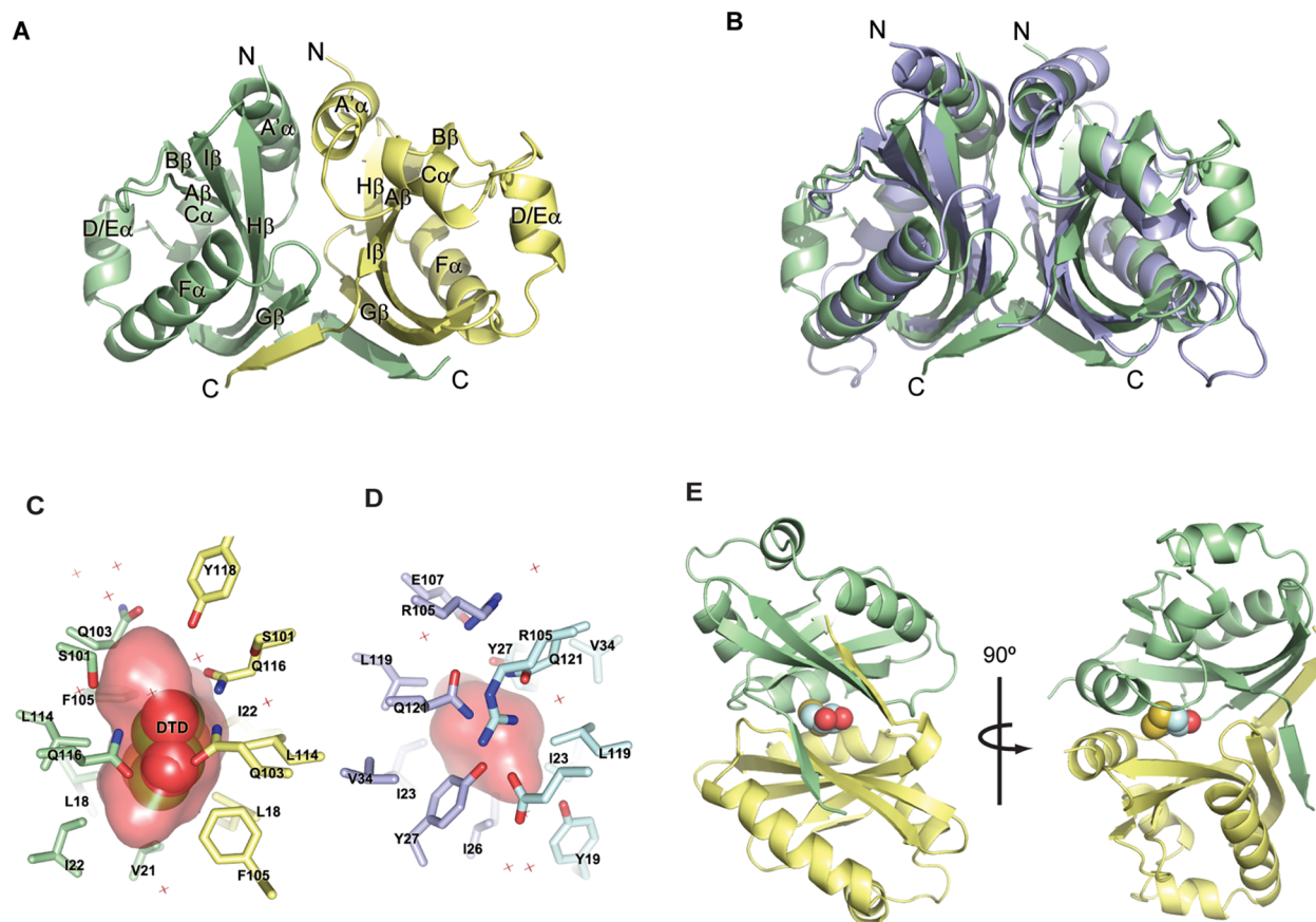
Figure 2. Homodimerization of TraJ 11–130 and TraJ pSLT 1–128 . The two protomers of each dimer are colored differently. (A) Crystal structure of a TraJ 11–130 dimer. (B) Superposition of the TraJ 11–130 (green) and TraJ pSLT 1–128 (blue) dimers. (C) TraJ 11–130 residues surrounding DTD (shown as spheres) at the dimeric interface. The surface of the internal pocket is colored red. (D) Residues surrounding a small cavity at the dimeric interface of TraJ pSLT 1–128 . (E) Position of the DTD (spheres) pocket in the overall structure of a TraJ 11–130 dimer.
