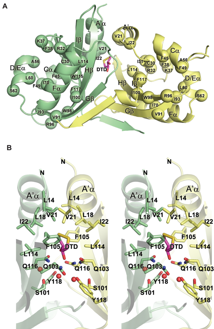
Figure 3. Functionally deleterious mutations in TraJ F 11-130 reveal conserved structural components. (A) Mapping of deleterious missense mutations (spheres) onto the TraJ F 11-130 dimer. The two protomers are colored green and yellow. See Figure S1 of the Supporting Information for the identity of the missense mutations. (B) Stereoview of the dimerization interface of the TraJ F PAS domain formed by interactions between the N-terminal helices (A'α) and the β-sheets from both protomers. Water molecules are represented by red spheres.
