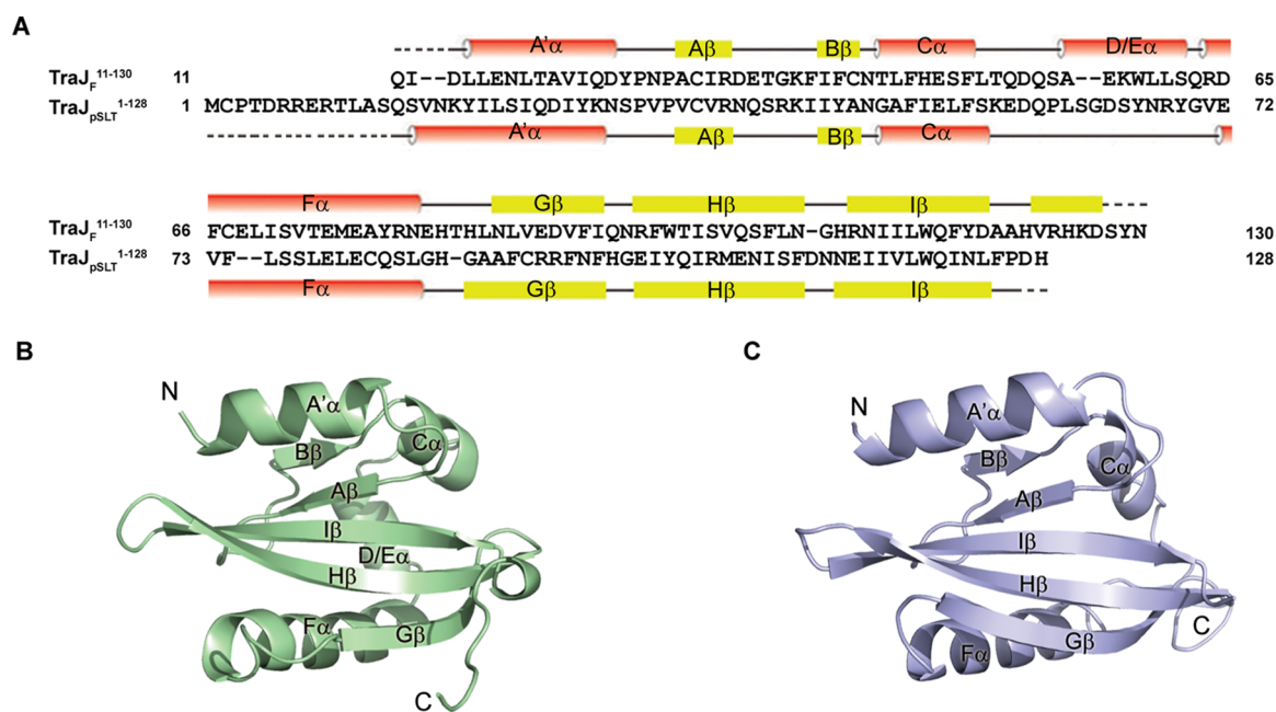
Figure 1. Overall structures of TraJ F 11-130 and TraJ P SLT 1-128 . (A) Alignment of amino acid sequences of TraJ F 11-130 and TraJ P SLT 1-128 . Secondary structure elements of TraJ F 11-130 and TraJ P SLT 1-128 are shown above and below the corresponding sequences, respectively. Dotted lines indicate residues not modeled in the crystal structures because of a lack of electron density. (B) Crystal structure of a TraJ F 11-130 monomer. Secondary structural elements as well as the N- and C-termini are labeled. (C) Crystal structure of a TraJ P SLT 1-128 monomer.
