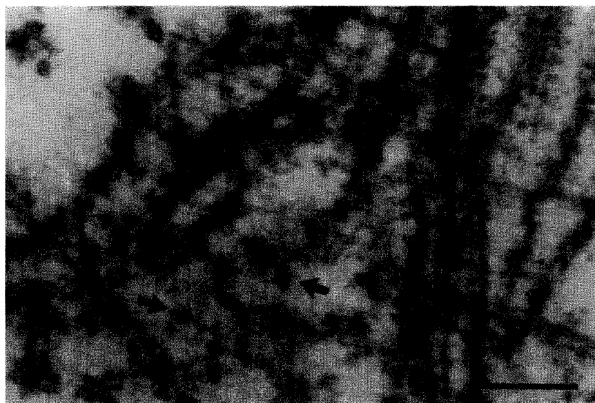
FIGURE 4. Transmission electron micrograph of deposits between rejecting Botryllus oozoids. The 150–200-angstrom-wide fibers are double tracked and show a regular periodicity of structure suggestive of stacked subunits. Fibers crossing the plane of section head on are pentameric or hexameric with a central hole, similar in shape and size to the larger HA-1 discs in Fig. 1 and to stacked SAP (Pepys et al., 1978). The bar spans 1500 nm.
