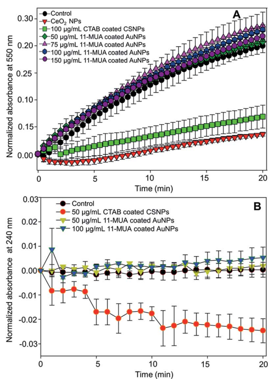
Fig. 8 SOD and catalase-like activity of CTAB coated CSNPs and 11-MUA coated AuNPs: time dependent SOD-like activity of CTAB coated CSNPs (100 μg mL -1 ) and different concentration of (50, 75, 100, and 150 μg mL -1 ) of 11-MUA coated AuNPs was measured by the reduction of ferri-cytochrome C by superoxide anions and measuring the absorbance at 550 nm (A). Time dependent catalase enzyme-like activity was measured by following the decrease in absorbance of H 2 O 2 at 240 nm exposed to CTAB coated CSNPs (50 μg mL -1 ) and 11-MUA coated AuNPs (50 and 100 μg mL -1 ) was recorded by UV-Visible spectrophotometer (B). Data expressed as standard deviation calculated from 3 experiments.
