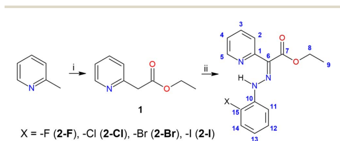
Scheme 1 Reaction scheme for the preparation of compounds 1 , 2-F , 2-Cl , 2-Br , and 2-I ; (i) lithium diisopropylamide (2.05 eq.), diethyl carbonate (3 eq.), THF, Ar, –84 °C; (ii) (1) 2-halogen aniline, NaNO 2 (1.1 eq.), HCl, H 2 O, 0 °C, (2) 1 , NaOAc (9 eq.), EtOH, H 2 O, 0 °C.
