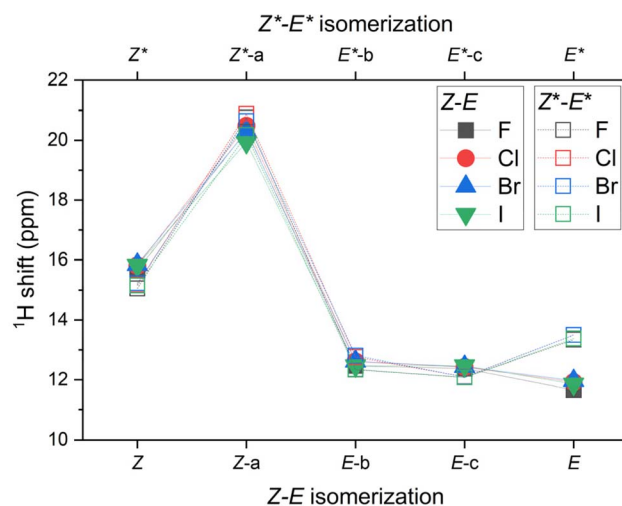
Fig. 5 The variation of ^1\text{H} NMR shifts along Z\text{-E} ( Z^*\text{-E}^* ) pathway for the hydrogen atom bonded either to azo-group or to pyridine moiety of 2\text{-X} compounds based on CAM-B3LYP/pcSseg-2/C-PCM( \text{CHCl}_3 ) calculations.
