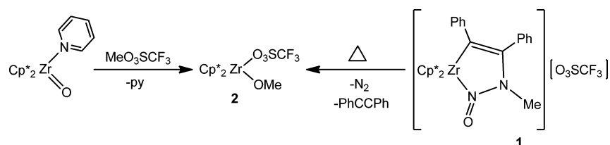
Scheme 5. Alkylation of the Azoxymetallacyclobutene Complex Cp* 2 Ti(N(O)NCPPhCPh) with MeO 3 SCF 3 to Form an Equal Mixture of 3 and 4
