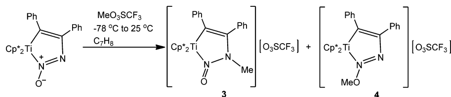
Scheme 5. Alkylation of the Azoxymetallacyclobutene Complex Cp* 2 Ti(N(O)NCPPhCPh) with MeO 3 SCF 3 to Form an Equal Mixture of 3 and 4
