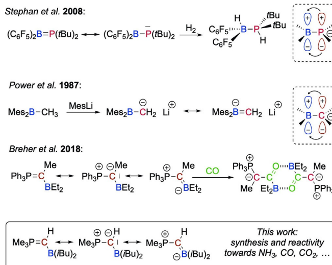
Scheme 1. Structures and reactivity of selected heteroalkenes. Mes = mesityl.
