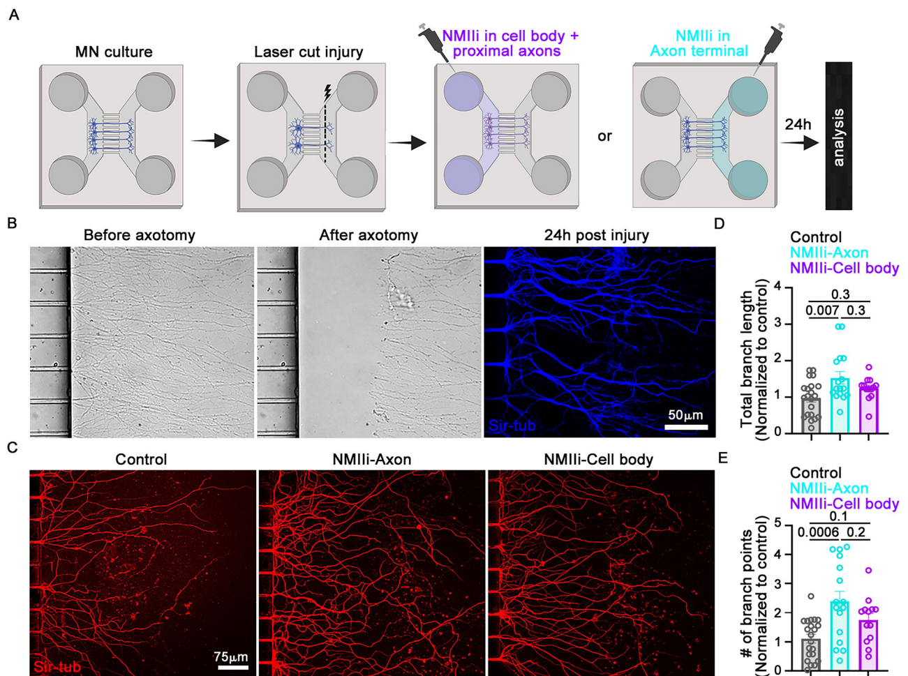
Fig. 4 | NMII inhibition of injured axons increases neurite length and branching. A Schematic of local NMII2 incubation of motor neuron cell bodies/proximal axons or distal axons in a microfluidic device and of the site of the axonal injury, by BioRender. Zeng, X. (2025) https://BioRender.com/i63w966 . B Images of neuronal projections passing across microfluidic device microgroove before and after axotomy. Regenerating axons labeled by Sir-tub 24h-post injury (C) Representative images of regenerated axons incubated with DMSO, 10 \mu M NMII2 in either the axonal or cell body site for 24 h after a laser cut axonal injury. Images by confocal
