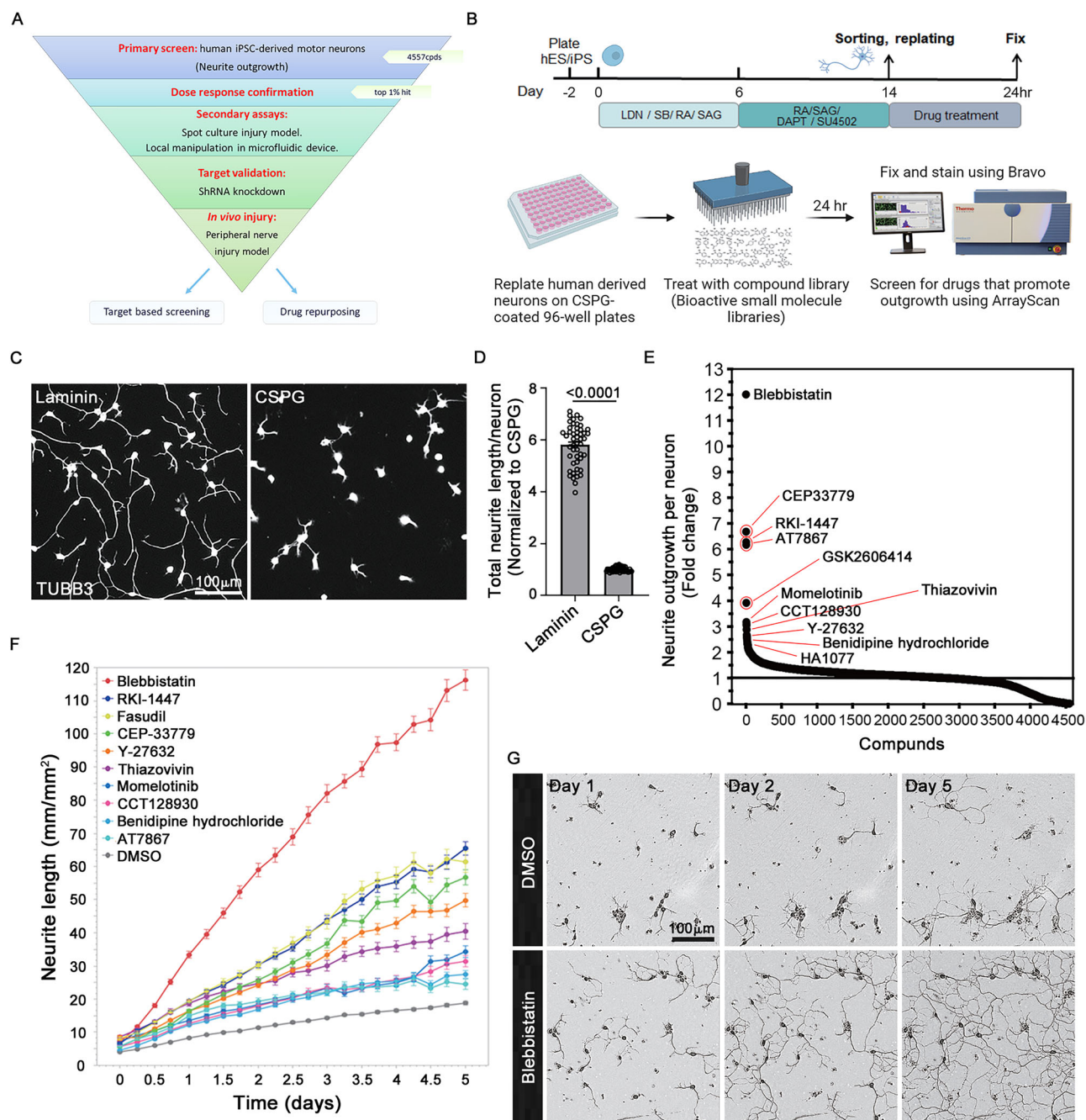
Fig. 1 | High-throughput phenotypic screening platform with human iPSC-derived motor neurons to identify pro-regenerative compounds. Screening funnel illustrating the screening strategy (A), and a schematic of the primary compound screen strategy (B), illustrated by BioRender. Zeng, X. (2025) https://BioRender.com/f56i717 . Human iPSC-derived MNs, after replating in 96 well plates, were cultured for 24 h on laminin or CSPG and stained with an antibody against TUBB3 (C). Quantification of total neurite length per neuron on the growth substrates, normalized to CSPG (D). Experiments were done in two biological replicates and analyzed from 48 technical replicates per group. Statistics, unpaired two-tailed t test, SEM error bars, and p -value: < 0.0001. Data is available in the Source
