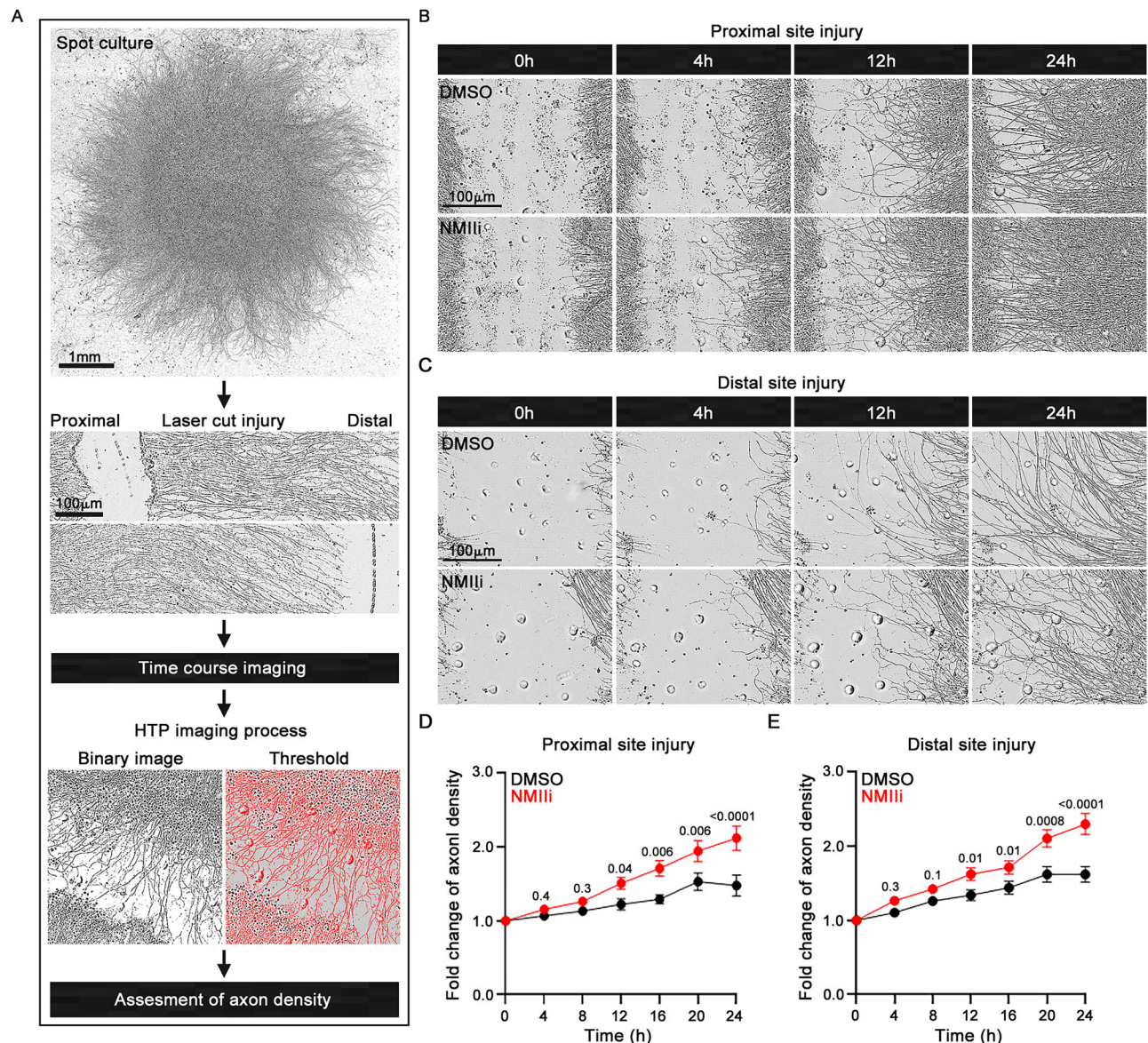
Fig. 3 | NMII inhibition promotes regeneration after axonal injury. A Image of a day 7 spot culture of human motor neurons with neurites projecting unidirectionally from cell bodies in the center. A laser cut injury was applied ~200 \mu m from the edge of the cell body cluster (proximal site injury) or ~700 \mu m from the cell body cluster, near the axon terminals (distal site injury). Injury size: 200–300 \mu m. Axon density was measured using a high-throughput SNT script that crops the injury site, adjusts the threshold, and binarizes the raw images. Images of regenerating neurons after axonal injury at proximal ( B ) or distal ( C ) sites. Scale bar: 100 \mu m. Quantification of axon density after a proximal ( D ) or distal injury ( E ) with DMSO or 10 \mu M NMIIi2. Experiments were in triplicates. Data from \geq 2 fields per spot were quantified and normalized to DMSO. All experiments conducted in triplicate,
