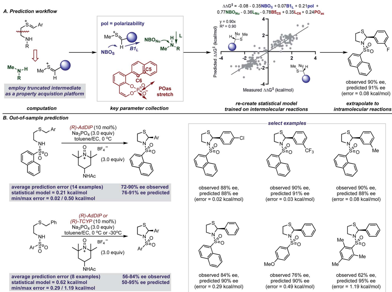
Fig. 7 (A) Comprehensive statistical modeling workflow that employs reaction \Delta\Delta G^\ddagger data from intermolecular reactions involving iminiums to predict reaction intramolecular reaction outcomes with thionium intermediates. A generic product denotes the stereochemical outcome predicted if the reaction proceeds through a -ee or +ee pathway and is catalyzed by the (R) -catalyst. Product stereochemistry is reversed if the opposite catalyst enantiomer is used. (B) Application to the formation of N,S -acetals.
