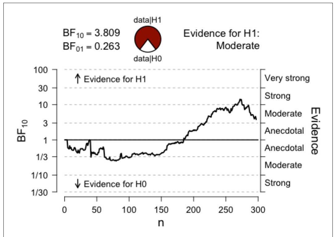
Figure 6. Sequential analysis. The graph shows the strength of evidence (as expressed by BF_{10} ) as N increases.
