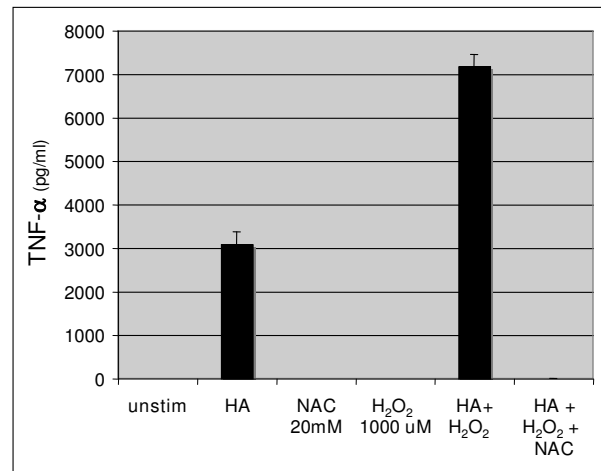
Figure 4 ROS synergize with HA fragments to induce inflammatory gene expression. ELISA for TNF- \alpha of cultured cell supernatants from MH-S cells stimulated with HA fragments (250 \mu g/ml) in the presence of H 2 O 2 (1000 \mu M) +/- NAC (20 mM) for 18 h. These data represent the average of 4 identical, independent experiments.
