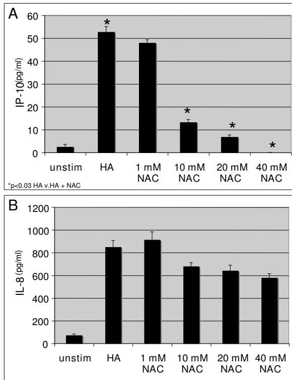
Figure 3 NAC inhibits HA fragment-induced gene expression in airway epithelial cells. ELISA for (A) IP-10 and (B) IL-8 of cultured cell supernatants from NCI H292 cells stimulated HA fragments (250 \mu g/ml) in the presence of NAC in concentrations as indicated at 37°C for 18 h. These data represent the average of 4 identical, independent experiments.
