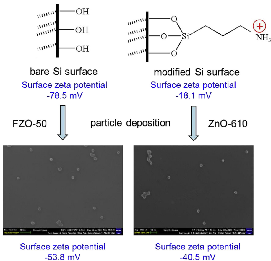
Fig. 6 – The change of surface zeta potential values before and after particle deposition. The magnifications of SEM images are 17.92\text{ k}\times (FZO-50) and 17.41\text{ k}\times (ZnO-610), respectively.
