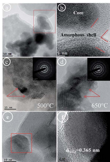
Fig. 5 HRTEM micrographs of: (a) Ti 2 La 2 O 7 precursor (low magnification), (b) Ti 2 La 2 O 7 precursor (high magnification), (c) Ti 2 La 2 O 7 and its FFT as inset, (d) Ti 2 La 2 O 7 and its FFT as inset. Red arrows show anatase grains, (e) high TEM magnification of selected area and (f) lattice fringes in HRTEM image of single NC.
