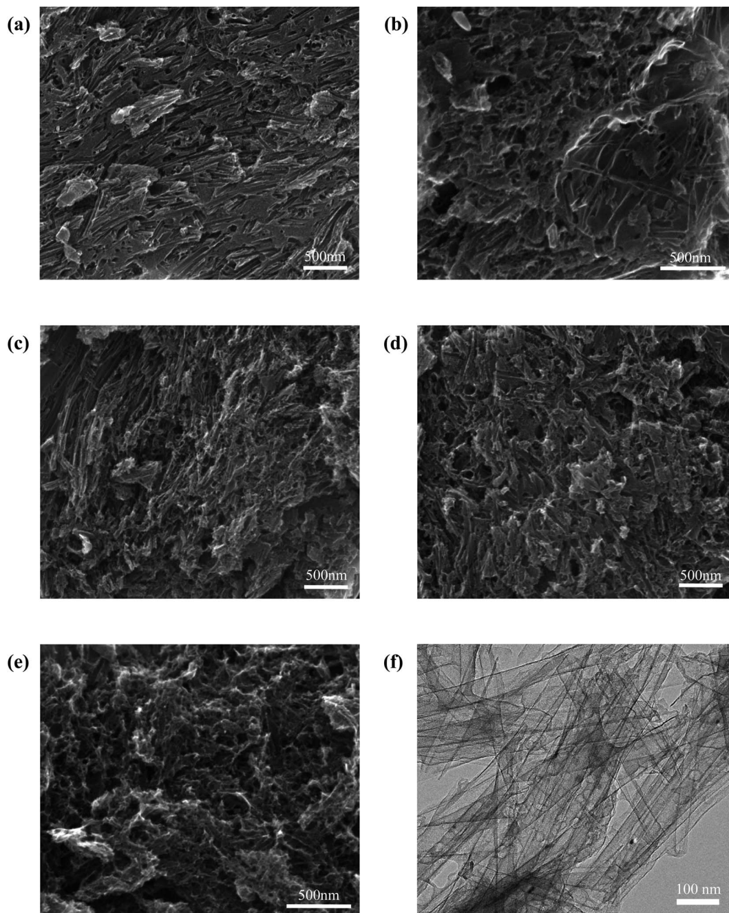
Fig. 4 Morphology of HTFBC and AHTFBC s . SEM images of (a) HTFBC; (b) AHTFBC 2 ; (c) AHTFBC 3 ; (d) AHTFBC 4 ; (e) AHTFBC 5 ; (f) TEM images of AHTFBC 4 .
