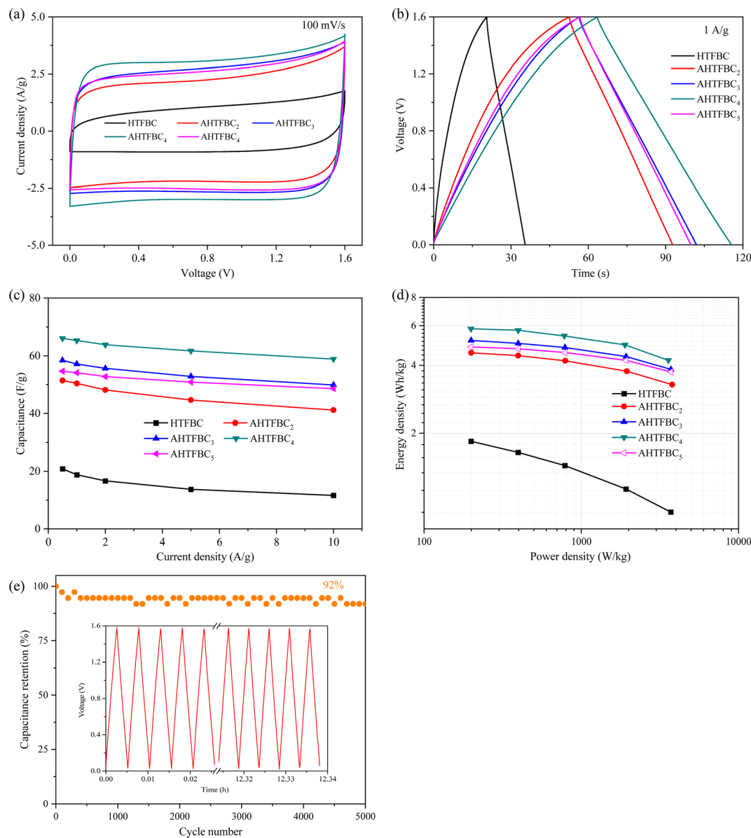
Fig. 8 Electrochemical properties of HTFBC//HTFBC and AHTFBC s //AHTFBC s symmetric supercapacitors in the 1 M Na 2 SO 4 electrolyte. (a) CV curves at 100 \text{ mV s}^{-1} ; (b) GCD curves at 1 \text{ A g}^{-1} ; (c) specific capacitances at 0.5\text{--}10 \text{ A g}^{-1} ; (d) Ragone plot; (e) cycling stability of AHTFBC 4 at 5 \text{ A g}^{-1} .
