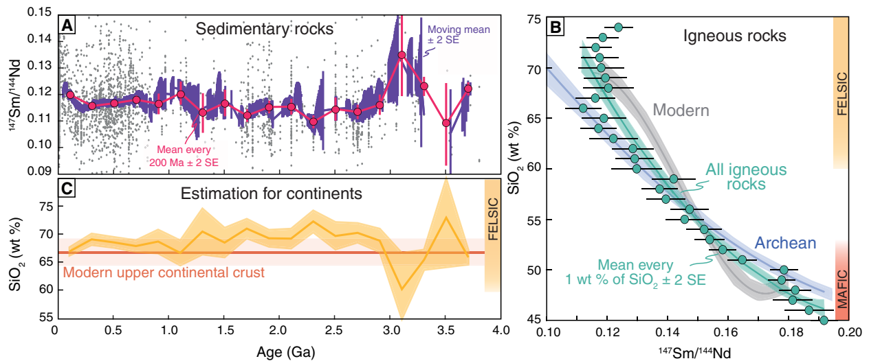
Fig. 1. Evolution of ^{147}\text{Sm}/^{144}\text{Nd} ratios and \text{SiO}_2 contents in rocks through time. (A) Compiled ^{147}\text{Sm}/^{144}\text{Nd} ratios of sedimentary rocks (gray points; data S1). Binned and moving means are shown in pink and purple with error bars. For the moving mean, the length of the sliding window is 200 Ma. The two types of means globally show the same variations through time. (B) Variation of \text{SiO}_2 contents as a function of ^{147}\text{Sm}/^{144}\text{Nd} ratios in Archean (blue), modern (gray), and all age (green) igneous rocks compiled from the GEOROC database. The best-fit regression lines are shown with 95% confidence interval (shaded areas). (C) Average \text{SiO}_2 contents of continents through time estimated using binned means in (A) and the correlation for all igneous rocks (green) in (B). Value for modern upper continental crust is from Rudnick and Gao (21).
