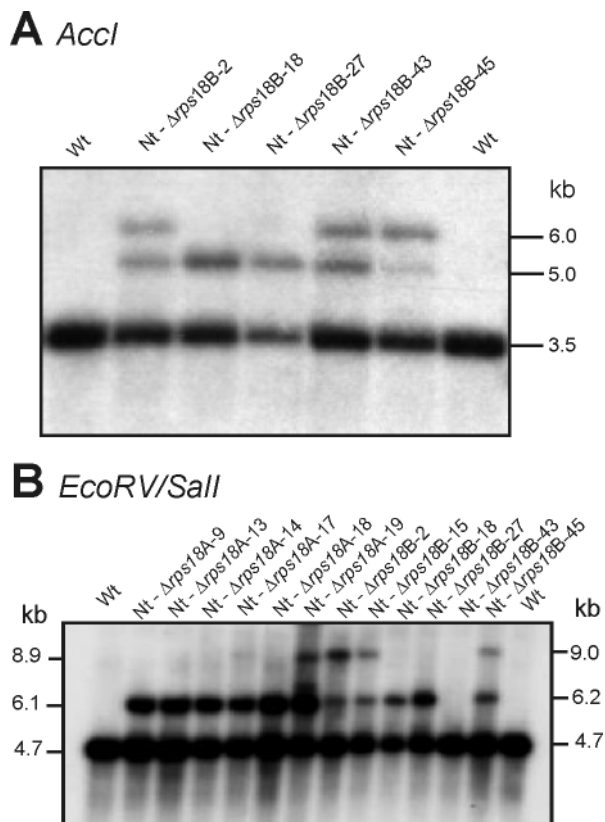
Figure 2. RFLP analysis of chloroplast transformants obtained with rps18 knockout constructs. Equal amounts of extracted total cellular DNA (5 \mu g per sample) were digested with the restriction enzymes indicated, separated in 0.8% agarose gels, blotted and hybridized to a radiolabeled restriction fragment derived from cloned tobacco plastid DNA (NdeI/SpeI fragment; Figure 1). (A) RFLP with AccI. (B) RFLP with EcoRV and SalI. The probe detects, in addition to the expected fragments (Figure 1), an unexpected band in most samples which is the product of flip-flop recombination (see text for details and Figures 3 and 4). Fragment sizes of the molecular weight marker are given in kb. Lane Nt- \Delta rps18B-43 is positive in the AccI RFLP and negative in the EcoRV/SalI RFLP most probably because the leaf sample harvested for DNA extraction for the AccI blot was heteroplasmic, whereas the sample harvested for isolating the DNA for the EcoRV/SalI blot had segregated into virtual homoplasmy for the wild-type genome. Wt: wild type.
