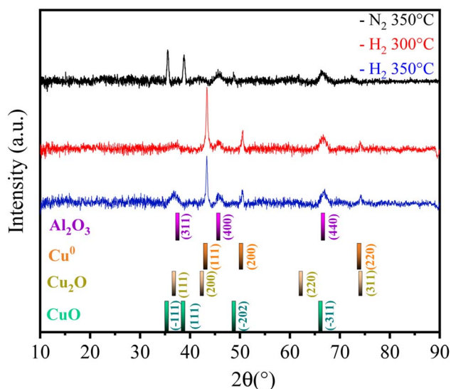
Fig. 6 X-ray diffractograms of Fe10Al190Cu catalyst after pre-treatment.
