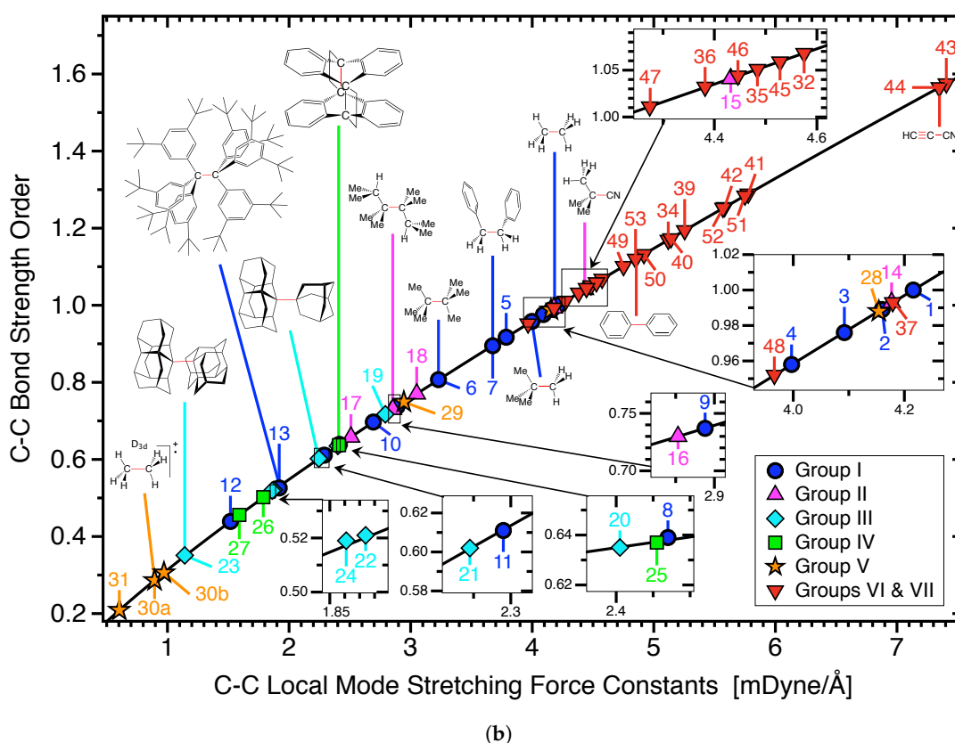
Figure 3. (a) BSO n values of all targeted CC single, double, and triple bonds for Group I-Group VII molecules, obtained with the power relationship BSO\ n = 0.3135\ (k^a)^{0.8062} utilizing local mode stretching force constants k^a (CC). Calculated at the \omega B97X-D/aug-cc-pVTZ level of theory. See text and Equation (6) for the derivation of the power relationship; (b) corresponding power relationship for all C–C bonds.
