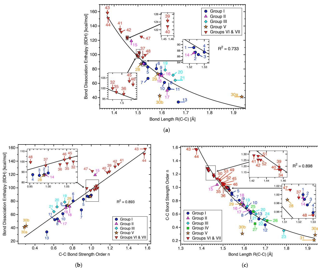
Figure 5. (a) Correlation between calculated bond dissociation enthalpies BDH_{calc} and calculated C–C bond lengths. BDH_{calc} values calculated with the composite G4 method and R(C–C) values at the \omega B97X-D/aug-cc-pVTZ level of theory; (b) correlation between BDH_{calc} and BSO n(C-C) . BDH_{calc} values were obtained using G4 and BSO n(C-C) values calculated at the \omega B97X-D/aug-cc-pVTZ level of theory; (c) Relationship between BSO n(C-C) and R(C–C) calculated at the \omega B97X-D/aug-cc-pVTZ level of theory.
