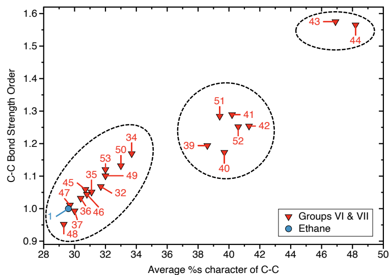
Figure 6. Average % s-character the targeted C–C bonds of ethane (1), Group VI, and Group VII molecules determined from the NBO analysis versus the corresponding BSO n(\text{C}-\text{C}) values. \omega\text{B97X-D/aug-cc-pVTZ} level of theory.
