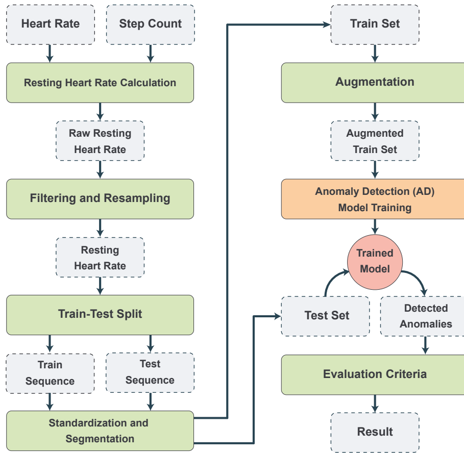
Fig. 2. Methodology overview of the anomaly detection framework using PCovNet.
