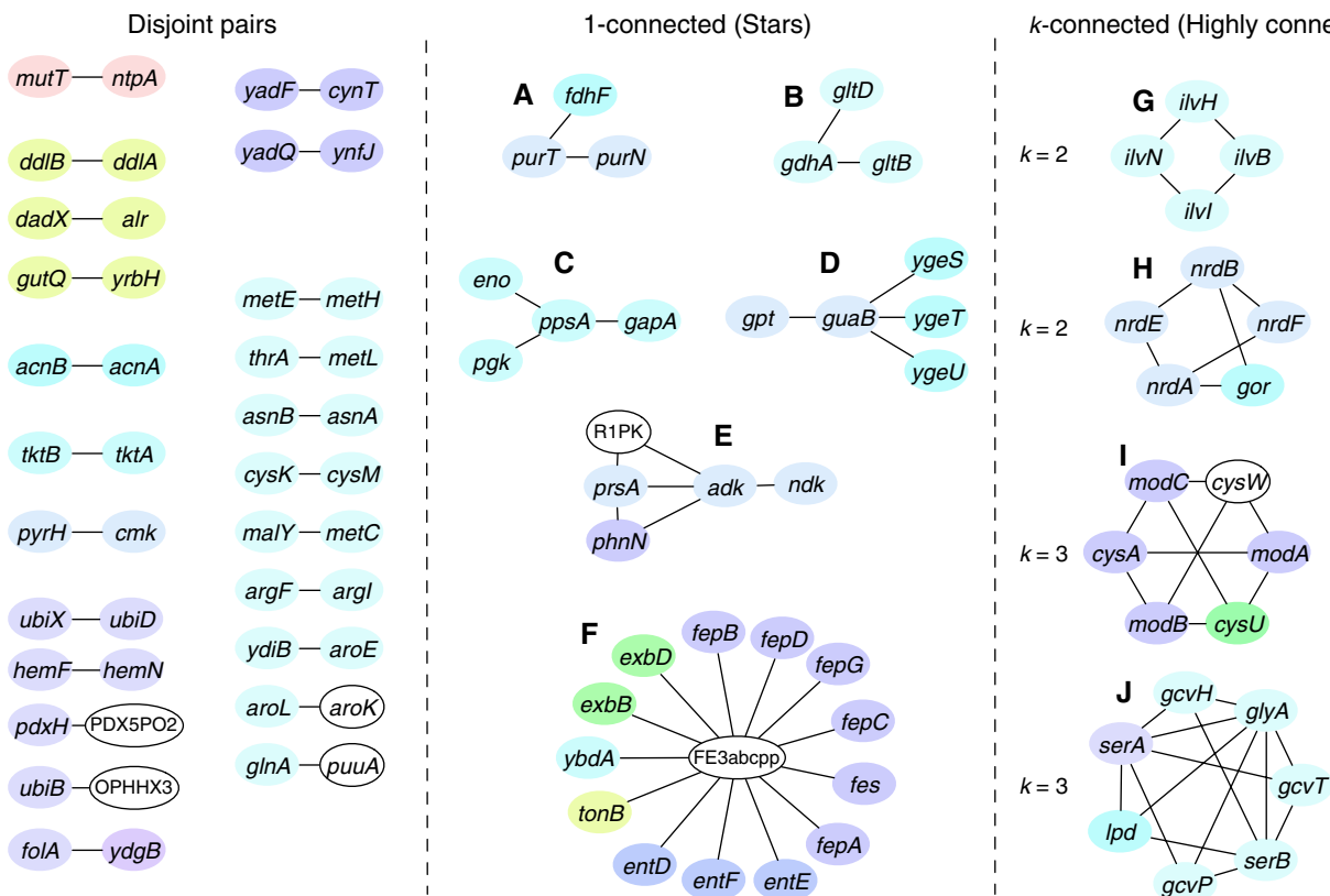
Figure 1 Topological and functional classification of clusters of SL gene pairs. Three types of network motifs are present: disjoint pairs (left); stars, or 1-connected motifs (center); and highly connected subgraphs, or k -connected motifs (right). Genes are color-coded in accordance to the COG (Tatusov et al , 2003) functional categorization. Names of genes are set in italics and the names of non-gene associated reactions are set in roman. Note that all the reaction abbreviations follow those in iAF1260 (Feist et al , 2007).
