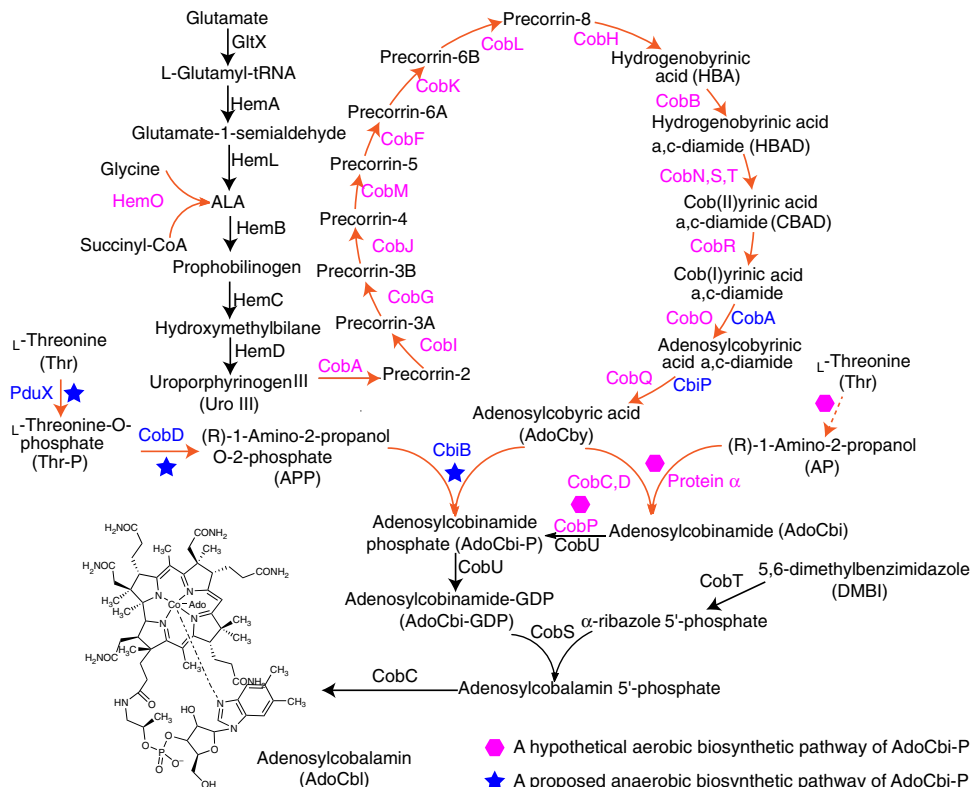
Fig. 1 Biosynthetic pathway of adenosylcobalamin. Endogenous enzymes from E. coli are shown in black. Enzymes from aerobic bacteria such as B. melitensis , R. capsulatus , S. meliloti , and R. palustris are shown in magenta. Enzymes from S. typhimurium are shown in blue. Ado represents the abbreviation of adenosyl
