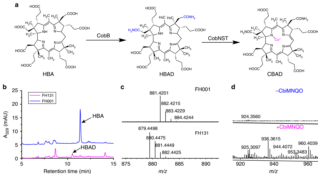
Fig. 2 The CBAD biosynthetic pathway and LC-MS detection of biosynthetic intermediates. a HBA is converted to CBAD by CobB and the CobN,S,T enzymes. b The strain FH131 expressing cobB converted HBA to HBAD, as assessed by HPLC. c Comparison of mass spectra for HBAD from the FH001 and FH131 stains. d Comparison of mass spectra for CBAD from recombinant E. coli stains with or without the expression of the cbiM,N,Q,O proteins
