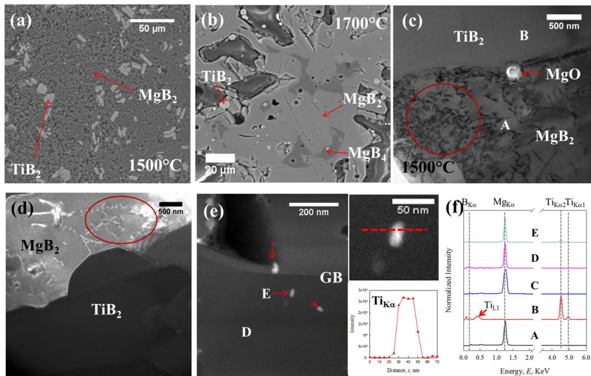
Figure 3. (a) BSE image of HTP-Ti-01; (b) BSE image of HTP-Ti-02; (c) BF TEM image of HTP-Ti-01. Large amount of crystal defects in \text{MgB}_2 grain close to \text{MgB}_2/\text{TiB}_2 interface; (d) DF TEM image of ingrain crystal defects in \text{MgB}_2 grain close to \text{TiB}_2 ; (e) HAADF image of \text{MgB}_2 grains with high defect density and STEM-EDS scanning across one of the nano-inclusions (red dash line). Inset is the intensity of \text{Ti}_{\text{K}\alpha} ; (f) EDS spectra of spot A-E from (c,e).
