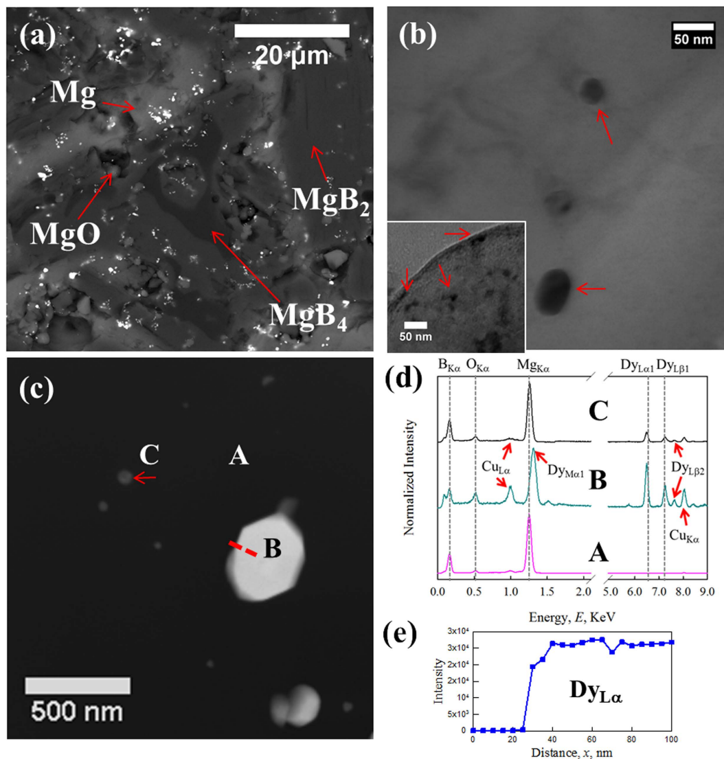
Figure 5. (a) BSE image of HTP-DY, four different phases ( \text{MgB}_2 , \text{MgB}_4 , Mg and MgO) are labeled; (b) BF TEM image of nano-size inclusions (10–50 nm) are found inside \text{MgB}_2 grains; (c) HAADF image of one \text{MgB}_2 grain, white precipitates are Dy-contained; (d) EDS spectra of spot A-C in (c); (e) the intensity of \text{Dy}_{\text{L}\alpha} from STEM-EDS scanning (red dash line in (c)).
