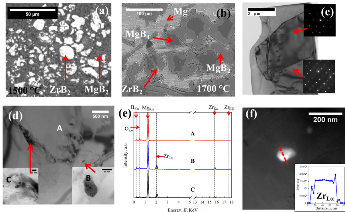
Figure 2. (a) BSE image of HTP-Zr-01; (b) BSE image of HTP-Zr-02; (c) BF TEM image of HTP-Zr-02 (Microstructures of the undoped bulk can be found in 6,18,19 ). Insets are SAD of two distinct \text{MgB}_2 grains; (d) nano-size inclusions observed close to/at \text{MgB}_2 grain boundaries; (e) EDS spectra of spot A, B and C; (f) HAADF image of a nano-size inclusion close to \text{MgB}_2 grain boundaries. Inset is the intensity of \text{Zr}_{\text{L}\alpha} from STEM-EDS scanning across the inclusion (red dash line).
