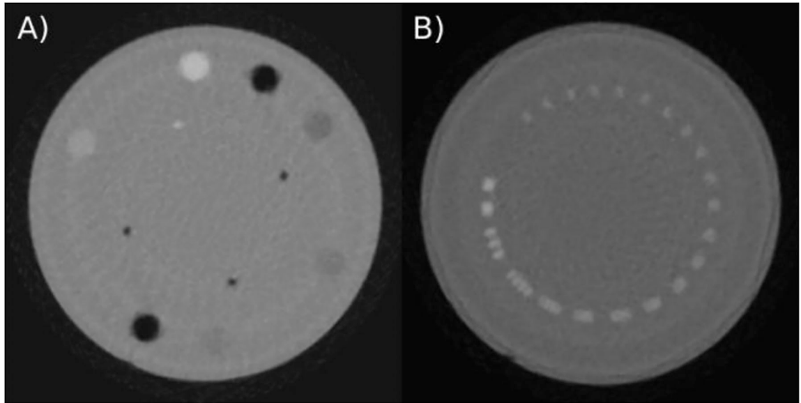
Figure 2: HeCT of A) the Catphan® CTP404 sensitometry module and B) the CTP528 high resolution module reconstructed using the DROP-TVS reconstruction algorithm with 512 \times 512 pixel per slice and slice thickness of 1.25 mm. The phantom was scanned 6 from 90 projections consisting of \sim 2.5 \times 10^6 particles each.
