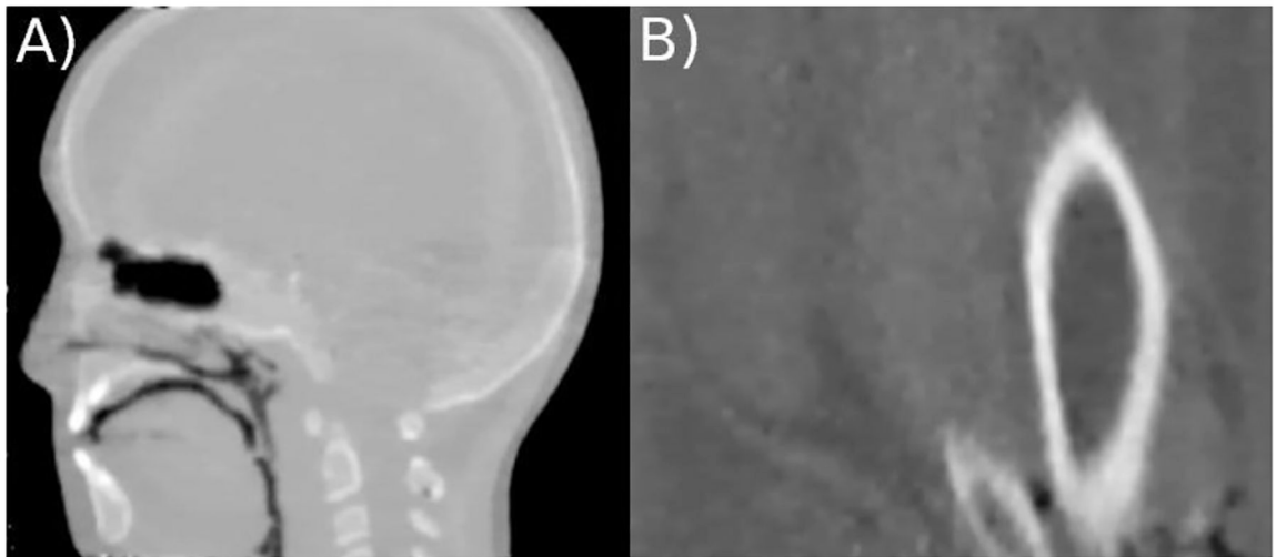
Figure 3: Vertical slice of a HeCT of A) the CIRS pediatric head phantom model HN715 (CIRS, Norfolk, Virginia, USA) and B) the custom build animal tissue phantom reconstructed using the DROP-TVS iterative reconstruction algorithm with 256 \times 256 pixel per slice and slice thickness of 1.25 mm. The phantom was 6 scanned using 90 projections consisting of \sim 4 \times 10^6 particles each.
