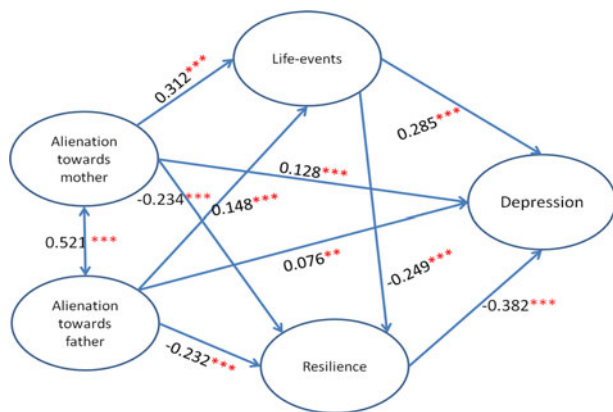
Fig. 1. AMOS structural equation model test for children's depression: Instant model.
