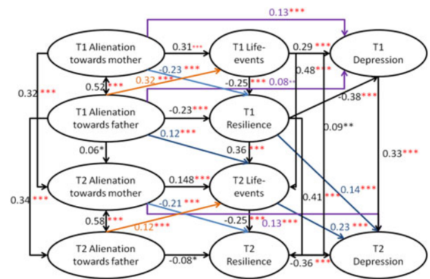
Fig. 2. AMOS structural equation model test for children's depression: Accumulated model.
