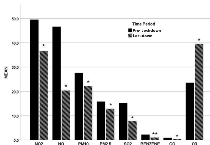
Figure 2. Mean air pollutants concentration in Lockdown and Pre- Lockdown period. All air pollutants are measured in \mu\text{g}/\text{m}^3 while CO is measured in \text{mg}/\text{m}^3 . One star (*) represents statistical significance at a level of 0.05, whereas two stars (**) at a level of 0.01.
