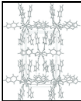
Fig. 2. Crystal packing of the title compound viewed along the c axis. Intermolecular hydrogen bonds are shown as dashed lines.
