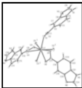
Fig. 1. The asymmetric unit of the title compound, showing 30% probability displacement ellipsoids. Symmetry code: (i) x, -y, 0.5+z .
