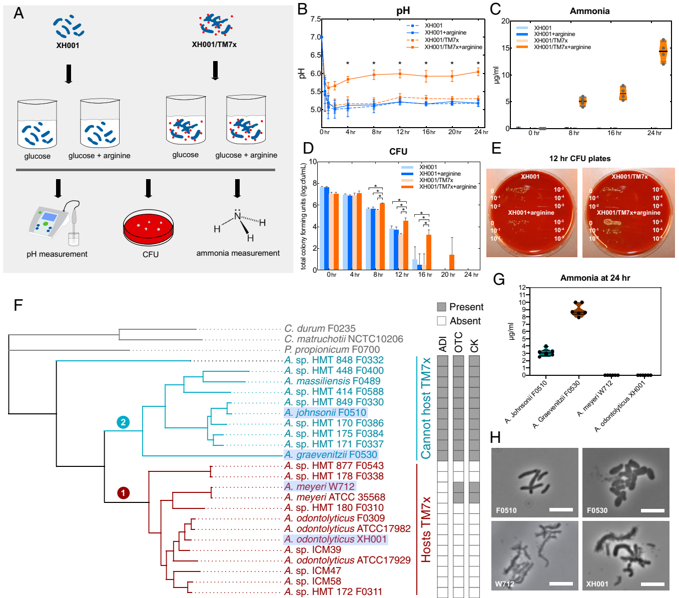
Fig. 4. TM7x-mediated pH buffering improves XH001 survival under acid stress which correlates with this strain only forming obligate associations with Actinomyces spp. lacking the ADS. (A) XH001 mono- and XH001/TM7x coculture were incubated in 0.85% NaCl + 10 mM glucose solution, supplemented with and without 10 mM arginine, a condition used for studying bacterial ADS function (23, 24). (B–E) pH of the solution (B), extracellular ammonia concentration (C), and XH001 viability (D and E) were monitored at the time points indicated ( Materials and Methods ). TM7x does not form a colony by itself. CFU data reflect only XH001 (D and E). Average values \pm SD are shown. A Kruskal–Wallis test (all pairwise, Bonferroni-adjusted) was used for statistical analysis; asterisks indicate significant differences between values ( *P < 0.05 ). (F) A phylogenetic tree was created using the 16S ribosomal RNA gene sequences of these oral Actinomyces spp. which revealed two clades: clade 1 (red) containing Actinomyces species capable of forming parasitic association with TM7x, and clade 2 (blue) including Actinomyces species unable to serve as host for TM7x based on experiments reported in ref. 28. The presence or absence of genes encoding the three key enzymes involved in the ADS pathway—ADI, OTC, and CK—within the genomes of these Actinomyces species is marked. (G and H) Two representative Actinomyces spp. from each clade (highlighted with light purple background) were chosen to test their ADS-mediated ammonia production (G) and TM7x infection (H). (G) Ammonia production after incubating A. johnsonii F0510, A. graevenitzii F0530, A. meyeri W712, and XH001 in saline supplemented with glucose and arginine for 24 h. (H) Phase-contrast images showing the non-TM7x hosts A. johnsonii F0510 and A. graevenitzii F0530, as well as the TM7x hosts A. meyeri W712 and XH001, during a TM7x infectivity assay. (Scale bars, 5 \mu m.)
