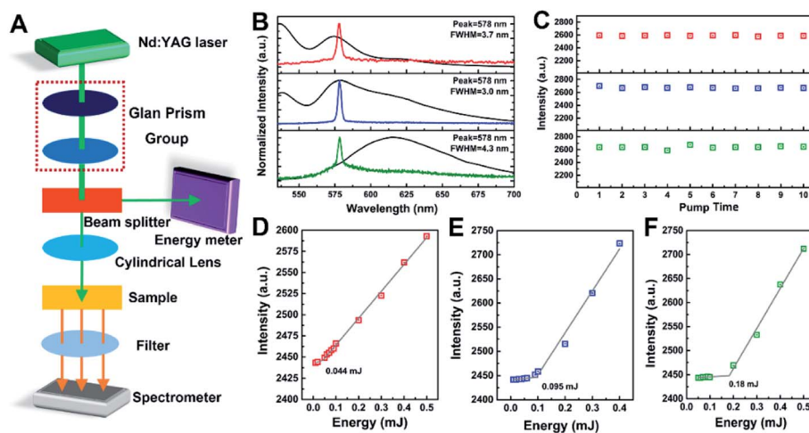
Fig. 5 (A) Schematic diagram for testing the emission properties by transmission mode. (B) Spontaneous emission (black lines, fluorescence) and stimulated emission (color lines, ASE) of hexylheptyl-PBI/PS film with different molecular aggregated states (red line: monomeric PBI, blue line: dimeric PBI and green line: oligomeric PBI), photo-pumped at 532 nm; (C) the ASE photostability of hexylheptyl-PBI/PS film with different molecular aggregated state (red line: monomeric PBI, blue line: dimeric PBI and green line: oligomeric PBI); (D and E) total ASE intensity emitted as a function of pump energy, a threshold behavior was observed for monomeric (D), dimeric (E) and oligomeric (F) dye.
