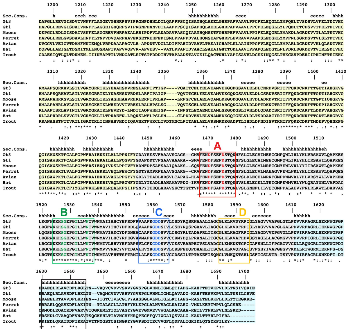
FIGURE 1 A conserved \alpha -helix is predicted in the thumb subdomain of the HEV RDRP. Sequence analysis of the RDRP domain of the HEV ORF1 protein. aa sequence alignment of the RDRP domains from a broad range of Hepeviridae family members (see details in Figure S2). A consensus secondary structure prediction (Sec. Cons.) for all sequences was determined on the basis of the algorithms DSC, GOR IV, HNN SIMPA96, PREDATOR, SOPM, and PHD available at https://npsa-prabi.ibcp.fr , as shown above the alignment (h, \alpha -helix; e, extended strand). Random coil or discrepant predictions are not indicated. The degree of aa physicochemical conservation at each position is shown on the bottom line and can be inferred from the similarity index according to ClustalW convention (asterisk, invariant; colon, highly similar; dot, similar). The fingers, palm, and thumb subdomains are denoted by light yellow, gray, and blue backgrounds, respectively. The conserved RDRP motifs A–D in the palm subdomain are indicated by colored boxes, and the fully conserved residues are highlighted in the same color. The predicted \alpha -helix in the thumb subdomain is highlighted by a black square. Numbering of aa is relative to the ORF1 protein sequence from HEV gt 3 strain 83-2-27 (AB740232) [Color figure can be viewed at wileyonlinelibrary.com ]
