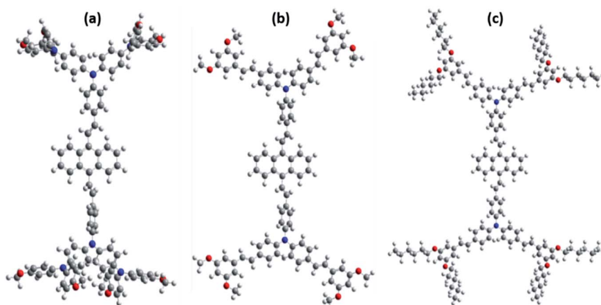
Fig. 2 Optimized structure of the anthracene based HTMs (a) ANTTPA, (b) AOME, and (c) AOHE.
