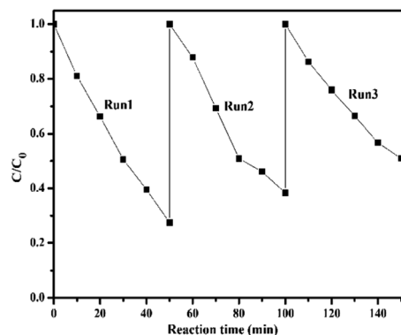
Fig. 2 Cycling runs in the degradation of BDE209 over BMO-5 in \text{N}_2 -saturated methanol system ( \lambda > 420 nm).
