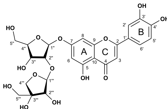
Fig. 4. Molecular structure of the isolated flavonoid 1 luteolin 7- O -[[ \beta -D-apiofuranosyl-(1 \rightarrow 2)- \beta -D-ribofuranoside].
